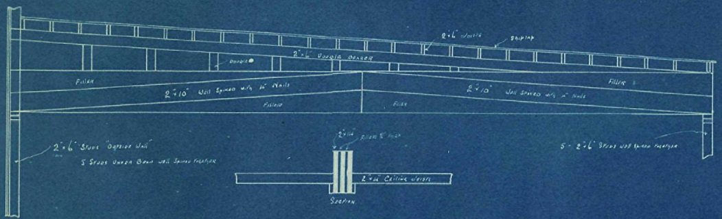
1/4 DETAILS of 4 TRUSSED BEAMS over Assembly Hall
