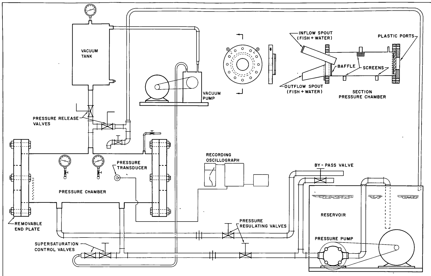
Figure 4. Diagrammatic representation of pressure apparatus.
