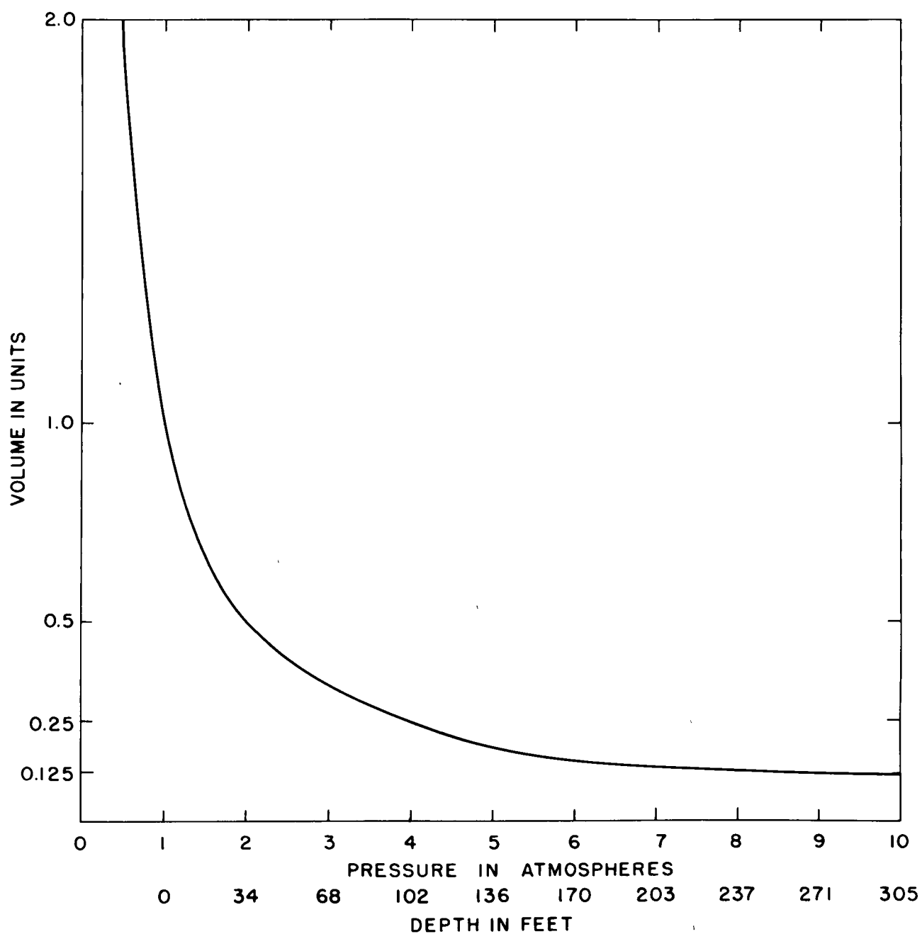
Figure 42. Change in unit volume of gas in relation to depth and pressure.
