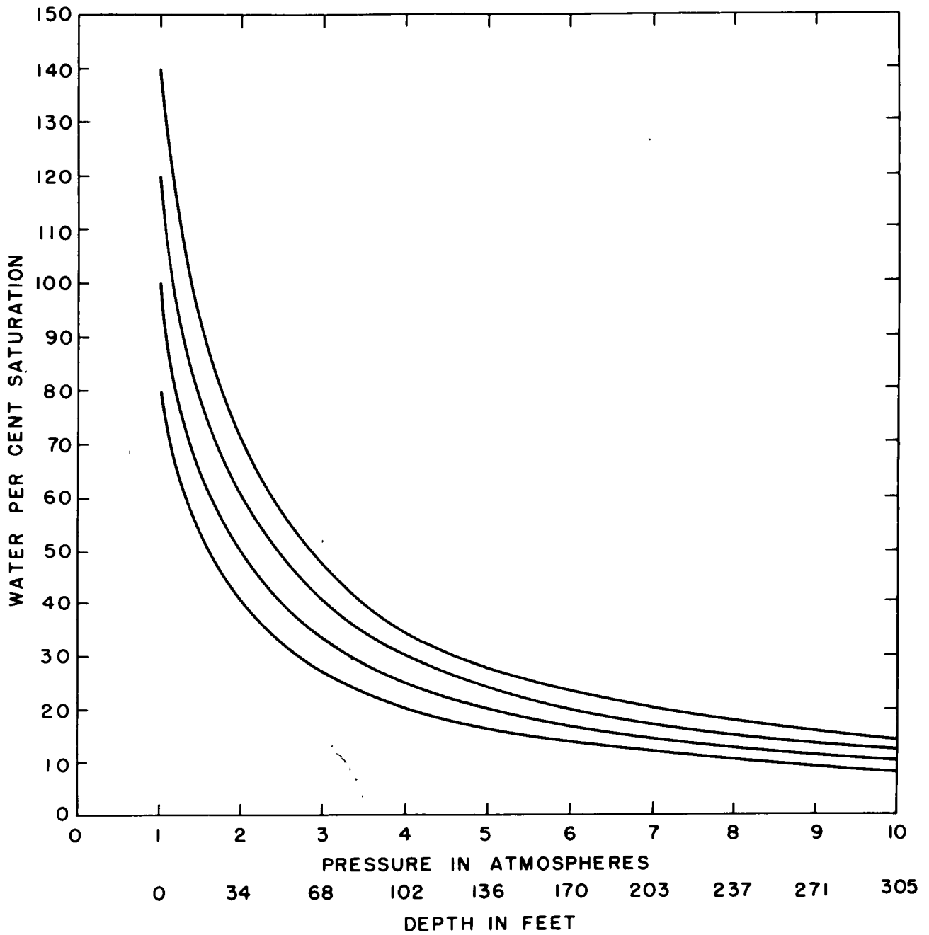
Figure 46. Per cent saturation in relation to pressure and depth. Absolute saturation of Ricker (1934).
