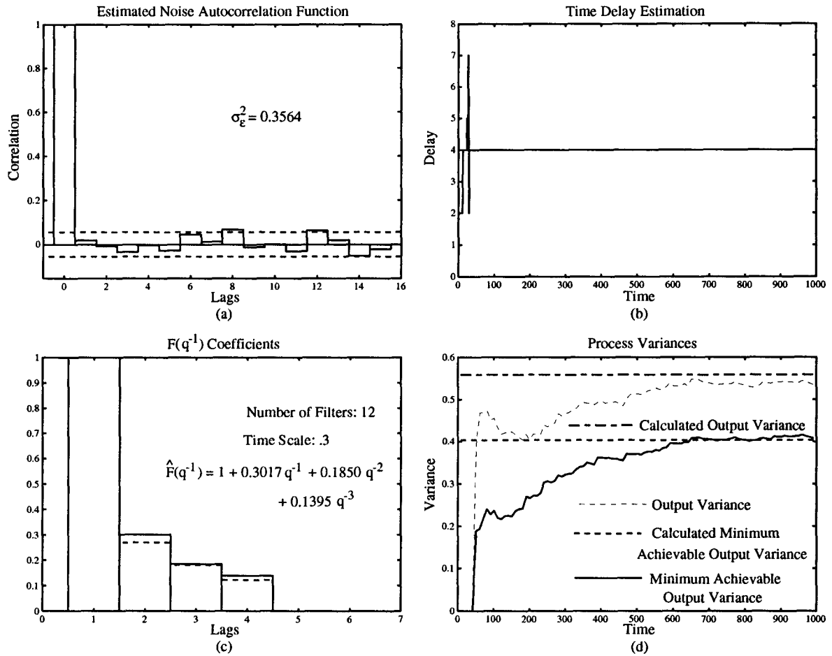
Figure 6.53: The (a) estimated noise autocorrelation function, (b) the FMVRE delay estimation, (c) the estimated F(q^{-1}) coefficients and (d) \hat{\sigma}_{mv}^2 and \sigma_v^2 for a change in plant
