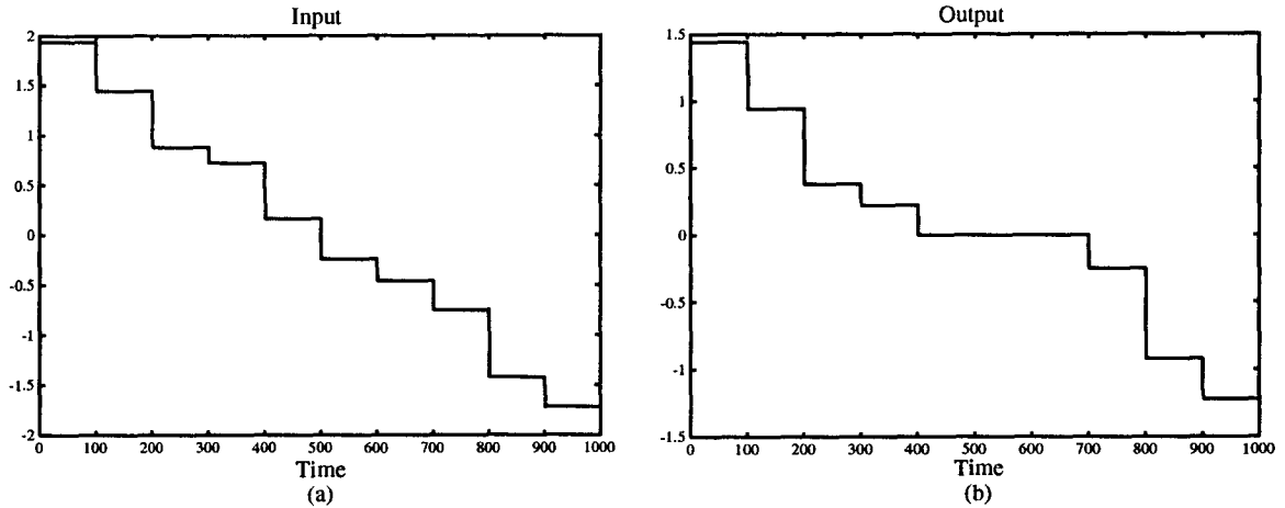
Figure 6.47: The (a) process input and (b) process output from the deadzone only
