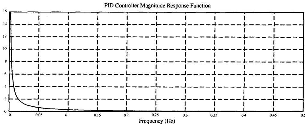
Figure 6.35: Magnitude response of the PID controller
