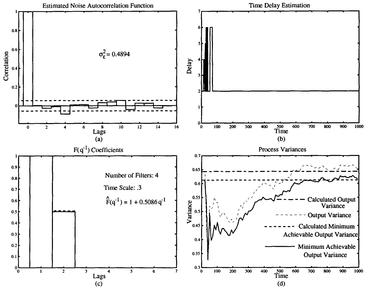
Figure 6.60: The (a) estimated noise autocorrelation function, (b) the FMVRE delay estimation, (c) the estimated F(q^{-1}) coefficients and (d) \hat{\sigma}_{mv}^2 and \hat{\sigma}_y^2 for process with real poles
