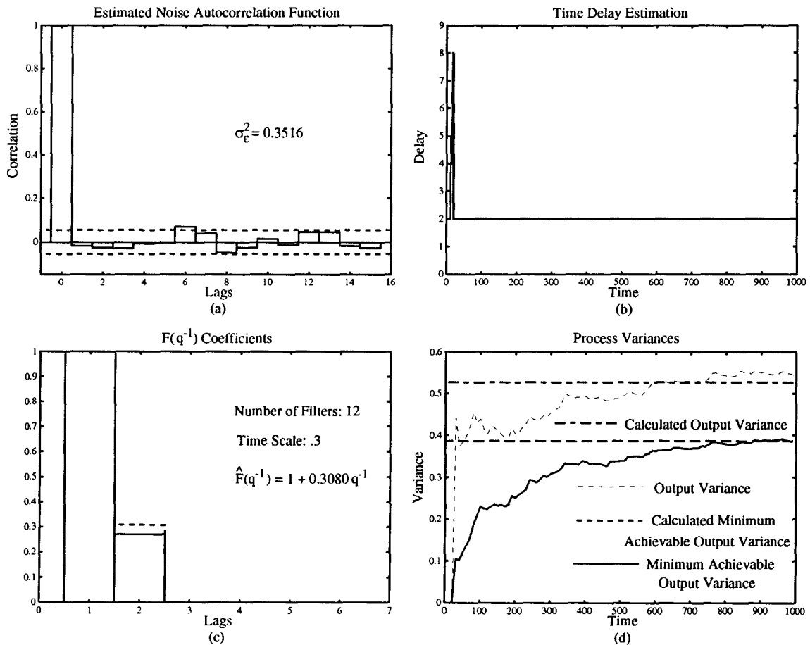
Figure 6.52: The (a) estimated noise autocorrelation function, (b) the FMVRE delay estimation, (c) the estimated F(q^{-1}) coefficients and (d) \hat{\sigma}_{mv}^2 and \sigma_y^2 for a change in delay
