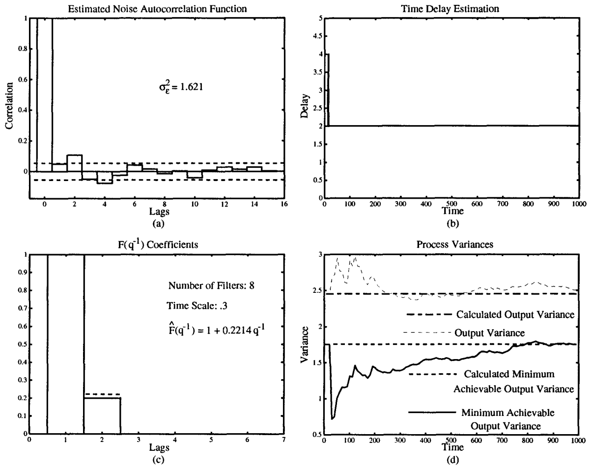
Figure 6.70: The (a) estimated noise autocorrelation function, (b) the FMVRE delay estimation, (c) the estimated F(q^{-1}) coefficients and (d) \hat{\sigma}_{\text{inv}}^2 and \sigma_y^2 for Dahlin controlled process with complex poles
