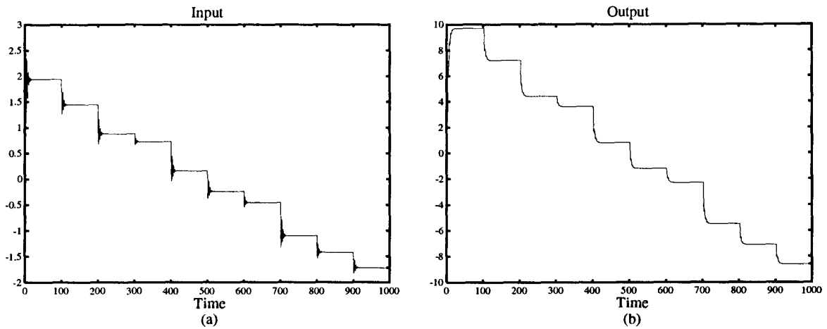
Figure 6.38: The (a) process input and (b) process output from closed loop operation
