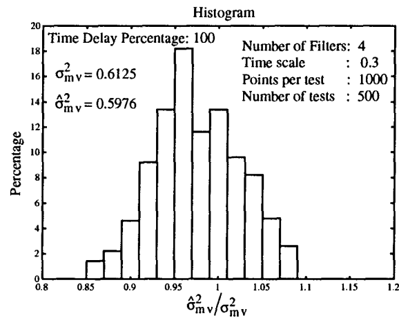
Figure 6.61: Distribution of the results of five hundred simulations for process with real poles
