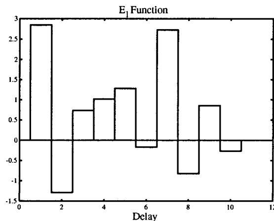
Figure 6.21: E_j function from FMVRE estimation resulting in a bias at one
