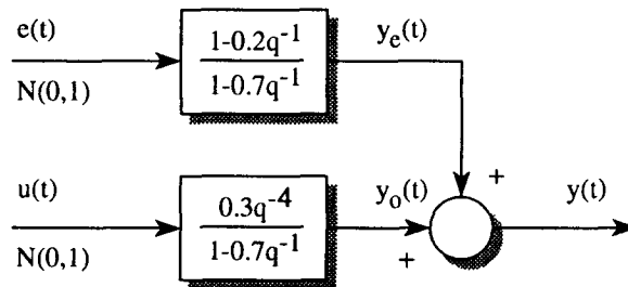
Figure 3.6: The stochastic process used for the example
