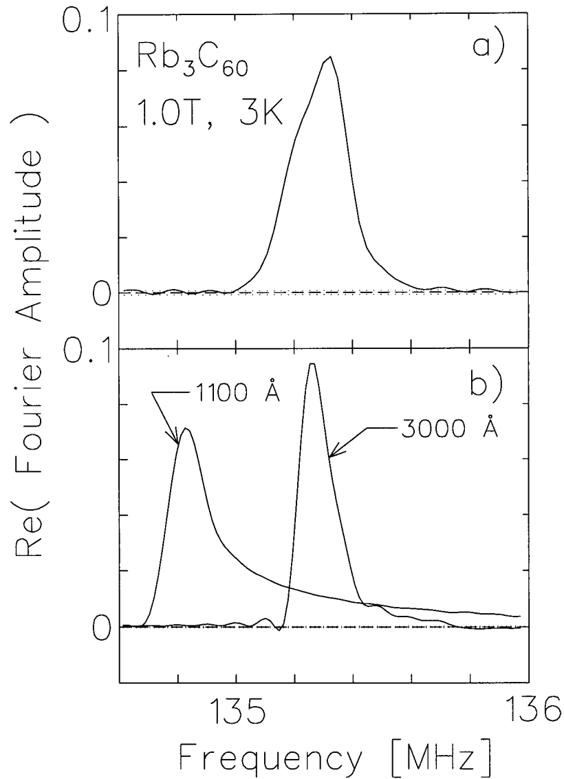
Figure 4.18: a) A high statistics \mu\text{SR} lineshape (FFT of TF asymmetry spectrum) in \text{Rb}_3\text{C}_{60} field-cooled to 3K at 1.0T applied transverse field. b) Simulated lineshapes for a perfectly ordered triangular flux-lattice using the Ginzburg-Landau theory.[191, 192, 193] The simulation parameters (\lambda, \xi) are (3000\text{\AA}, 30\text{\AA}) and (1100\text{\AA}, 30\text{\AA}) . The field distributions are convoluted with a Gaussian corresponding to the normal state linewidth. The 3000Å simulation also includes a small non-relaxing background signal known to exist in the data.
