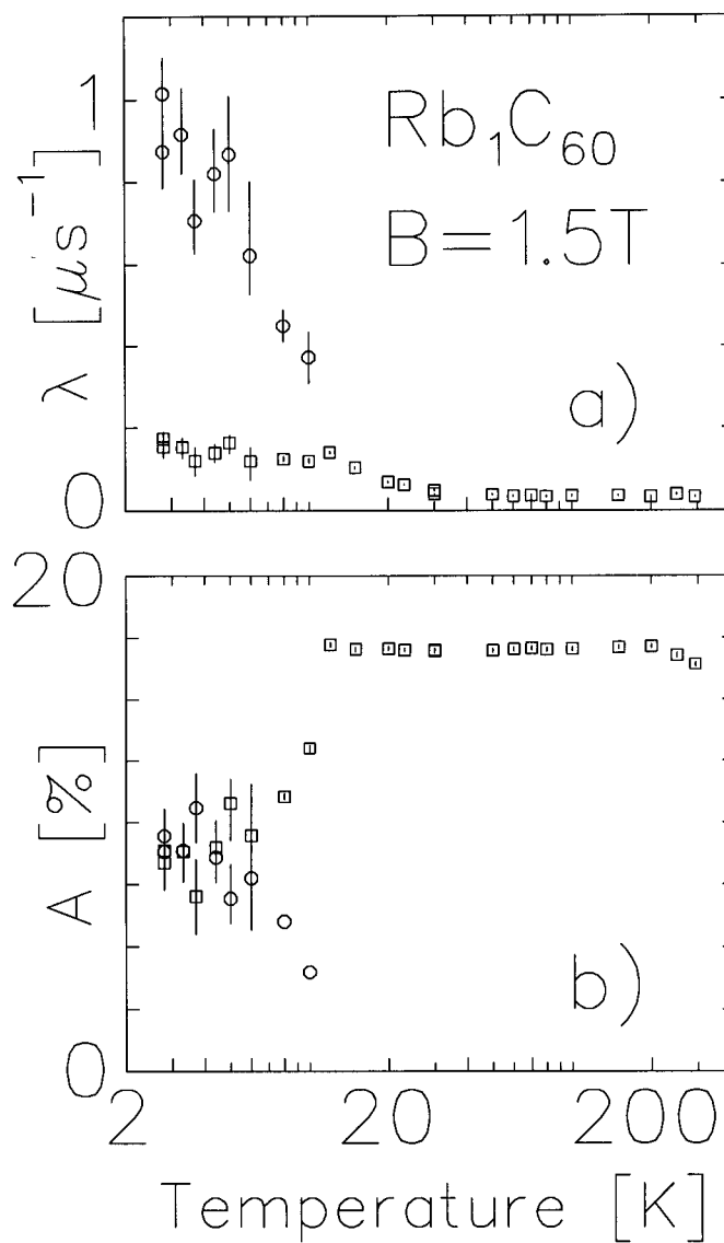
Figure 6.41: The a) exponential relaxation rates and b) corresponding amplitudes of the two relaxing signals from fits to the 1.5T TF relaxation. The third (non-relaxing) component was held fixed with temperature. Note the saturation to equal amplitudes of the two components.
