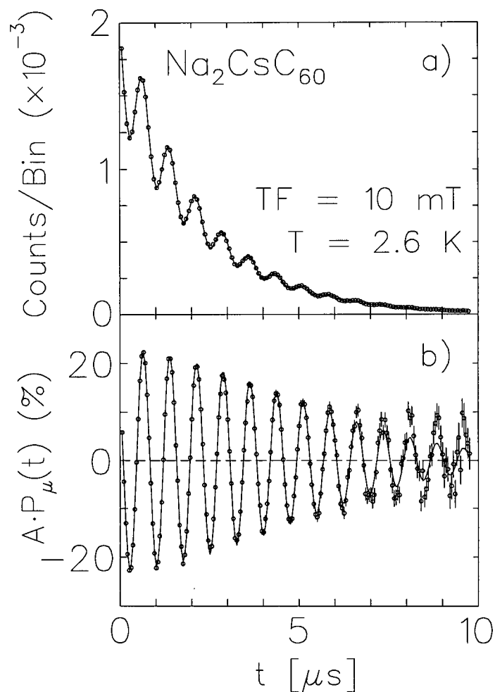
Figure 2.7: a ) The time histogram of muon-positron decays detected in a single counter in \text{Na}_2\text{CsC}_{60} in 10 mT transverse field (see Eq. (2.4)). b ) The same data combined with another histogram to remove the muon lifetime. A small non-relaxing signal, due to muons not stopping in the sample, is evident at late times. The relaxation is discussed in §4.2.
