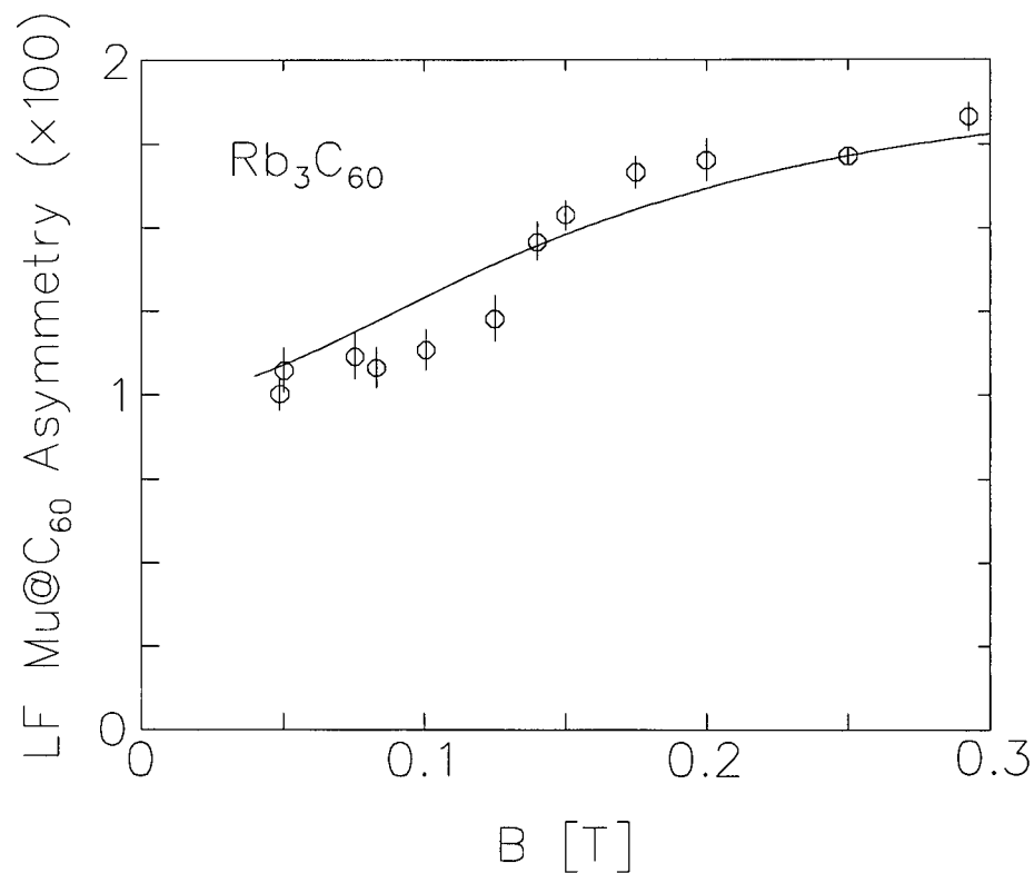
Figure 4.15: The LF dependence of the Mu@C 60 asymmetry (decoupling curve). The field at the inflection point indicates that the Mu hyperfine parameter is large (near its vacuum value). Each point is determined from a common fit to at least 2 different temperatures, ranging from 2.5 to 15 K (e.g. Fig.4.22).
