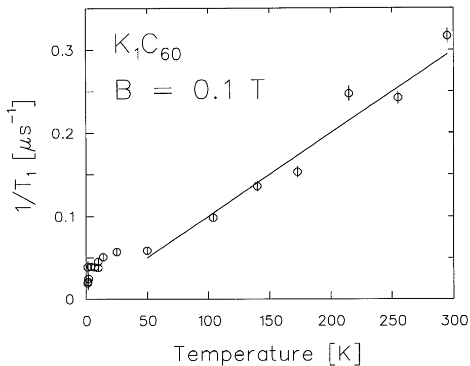
Figure 6.47: LF relaxation rate attributed to \text{Mu@C}_{60} undergoing fast spin-exchange with the conduction electrons in K_1\text{C}_{60} . The temperature dependence is not simply due to the Korringa mechanism as in A_3\text{C}_{60} , see text.
