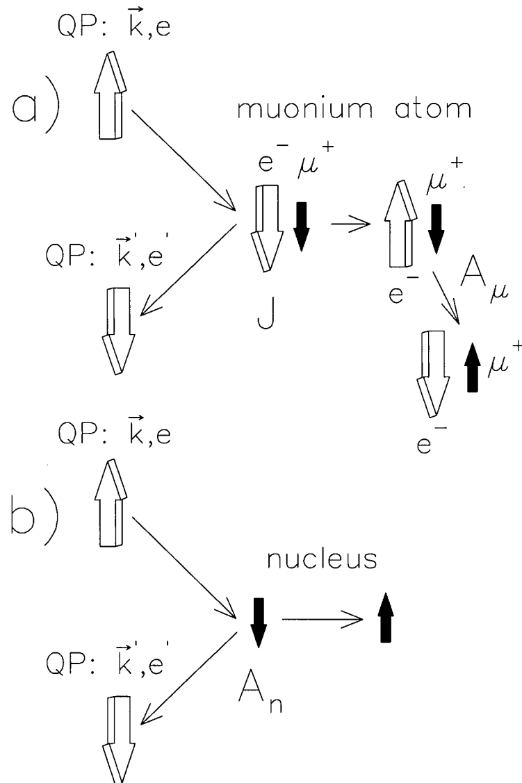
Figure 3.10: In each case a quasiparticle (QP) at the Fermi Surface with initial momentum \vec{k} and energy e scatters magnetically from the local moment. a) Spin exchange of a muonium atom (with subsequent evolution due to the muon-electron hyperfine interaction A_\mu ) vs. b) Electron-Nuclear spin-flip. In the spin exchange with the paramagnetic muonium, the electron Zeeman energies cancel; whereas in the latter, the nuclear and electron Zeeman energies do not.
