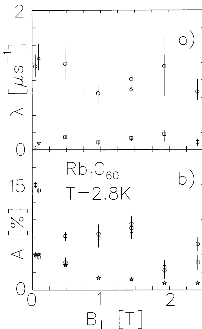
Figure 6.42: The a ) exponential relaxation rates and b ) corresponding amplitudes of the two relaxing signals from fits to the TF relaxation at 2.8K as a function of field. The triangles and nablas correspond to field cooled conditions, while the circles and squares are zero-field cooled. Because there was no significant effect of zero field cooling, these two cases have not been distinguished in panel b ). The third (non-relaxing) component was assumed to have the field dependence indicated by the stars in b ), in order to account for focussing of the muon beam.
