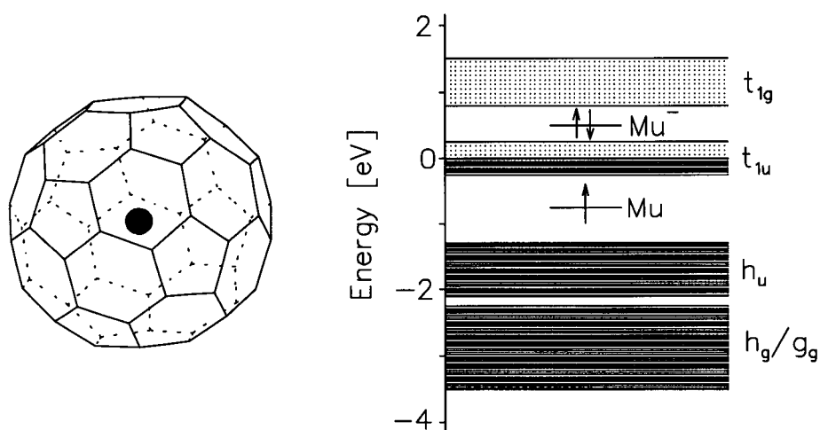
Figure 4.17: Proposed structure of \text{Mu@C}_{60} . The Mu atom is in the 1s ground state in the centre of the \text{C}_{60} cage. A large Coulomb energy is required to bind another electron to form \text{Mu}^- , so the \text{Mu}^- level may lie above the conduction band.
