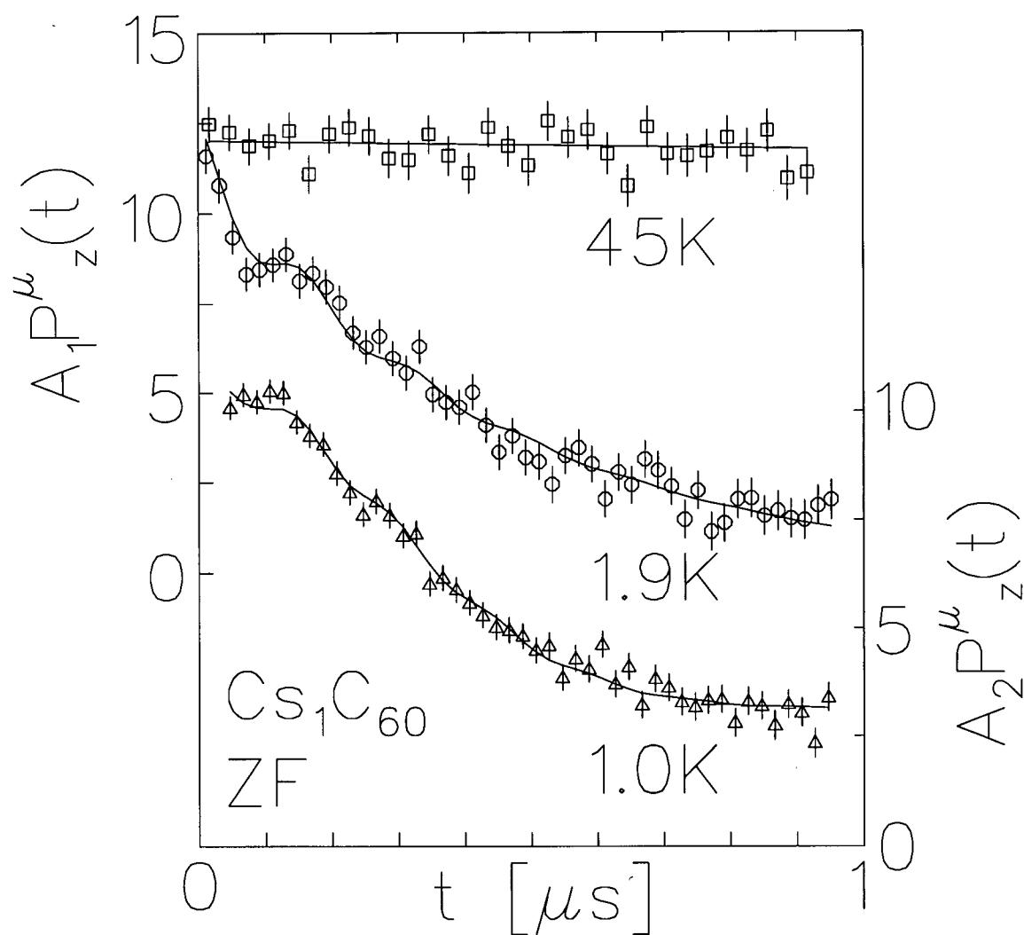
Figure 6.37: The fast component of the ZF relaxation in \text{Cs}_1\text{C}_{60} at the lowest temperature. There is a fast relaxing oscillation with a frequency of about 6MHz. The 45K data above the magnetic transition indicates that the fast component is not due to contamination from the early time straight through peak which does not occur in the sample spectra of the separate spectra apparatus.
