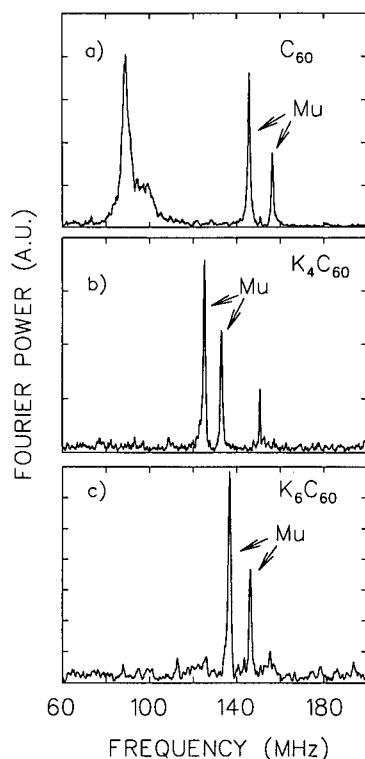
Figure 4.13: The TF precession signals of endohedral muonium in a) \text{C}_{60} at 10.7 mT, b) \text{K}_4\text{C}_{60} at 9.6 mT and c) \text{K}_6\text{C}_{60} at 10.0 mT (from Kiefl[14]). The broad line in \text{C}_{60} is due to the \text{C}_{60}\text{Mu} molecular radical, and the narrow line at 150 MHz in the \text{K}_4\text{C}_{60} spectrum is an instrumental effect. The frequencies and their field dependences correspond to vacuum-like Mu with A_\mu = 4341(24) , 4342(66) and 4230(63) MHz respectively.
