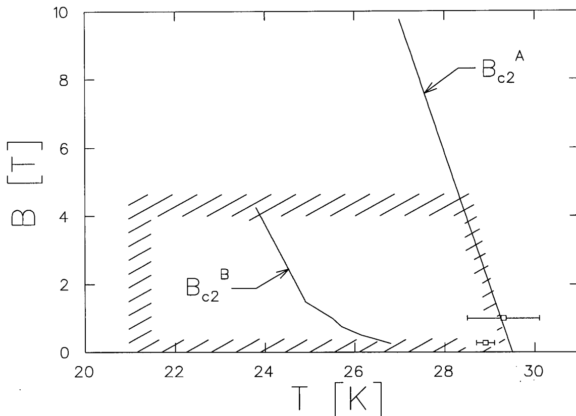
Figure 4.29: The H - T phase diagram of Rb_3C_{60} near T_c(0) \approx 29.5K . The curves are two different measurements of the upper critical field. The curve labelled A is from [31] and the curve labelled B is from [36]. The curvature of B is reminiscent of the “irreversibility line”, which separates the vortex liquid and solid phases. The hatched region is the region of the coherence peak measured by \mu\mathcal{SR} . The error bars are the measurements of T_c(H) from the TF \mu\mathcal{SR} (see Table 4.5) which are near curve A. Notice that the entire region of this diagram is contained in the extreme lower right corner of the generic phase diagram shown in Figure 3.12, so that the absence of the coherence peak expected in region (i) of Fig. 3.12 does not explain the observed damping which occurs at H/H_{c2}(0) \approx 0.1 .
