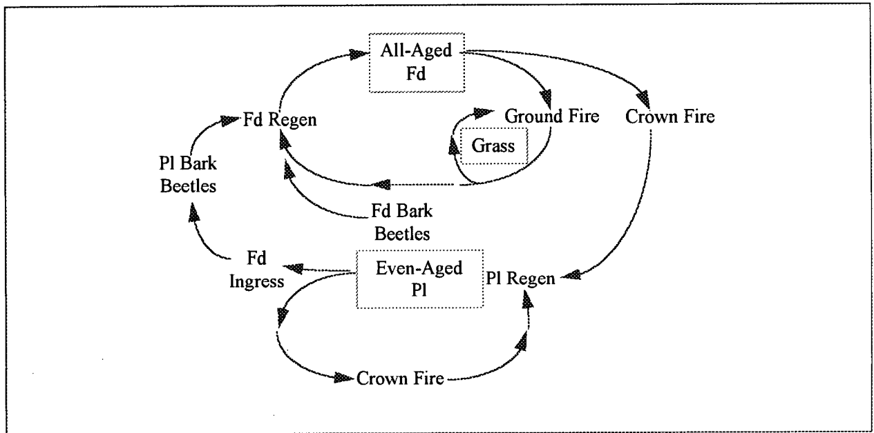
Figure 2: Gap dynamics (disturbance and succession) shift stands between grasslands, Douglas-fir (Fd) forests, and lodgepole pine (Pl) forests in the IDFdk3 at Knife Creek.
