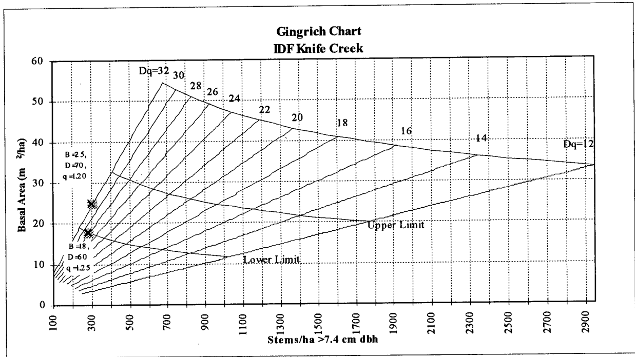
Figure 5: Gingrich Chart for Knife Creek after Day (1997b) indicating that the target stand for timber management (B=18, D=60, q=1.25) is at minimum stocking.
