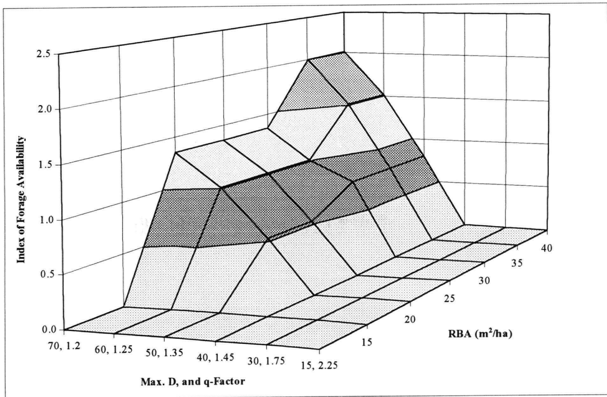
Figure 7: The impacts of target stand structure on an index of mule deer forage availability, suggesting that increasing RBA and Maximum Diameter improve forage availability.
