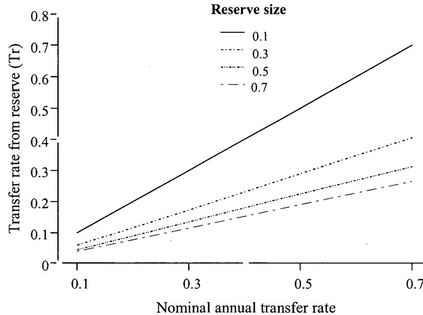
Figure 3.3 Behaviour of the transfer rates as a function of the size of the reserves.
