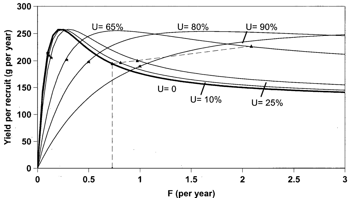
Figure 2.1 Yield per recruit for different size of unfishable areas ( U ) as a function of the fishing mortality on the harvested grounds (Redrawn from Beverton and Holt 1957). In order to evaluate marine reserves as a management tool the effort has been assumed to be concentrated on the harvested grounds, increasing F in fished areas. The broken line connects the yields for different reserve size corresponding to F_{\infty} = 0.73 , while the stars corresponds to F_{\infty} = 0.1 . See text for details.
