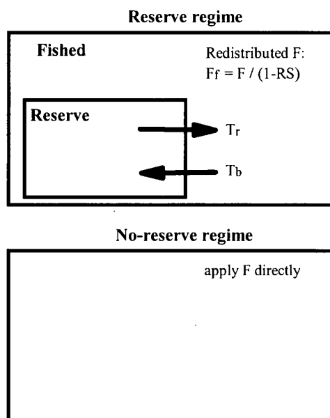
Figure 3.1. Organisation of the model. RS = reserve size as a proportion of the total area, F = instantaneous fishing mortality, F_f = redistributed F , T_r = transfer rate of fish from the reserve, T_b = transfer rate of fish from the fished area to the reserve, ref = reference reserve size (0.1), N_r and N_f = number of fish in the reserve and the fished area respectively.
