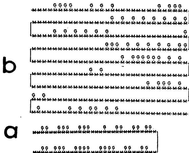
Fig. IV-2. Proposed structures for guaran (a) and locust bean gum (b) (from ref. 20).
