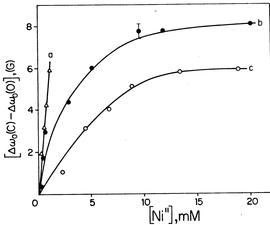
Fig. III-12. Plot of increase of centre-field linewidth of (a) [31], (b) [35], (c) [33] as a function of added nickel sulfate.
