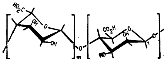
Fig. I-1. Structure of alginic acid.
