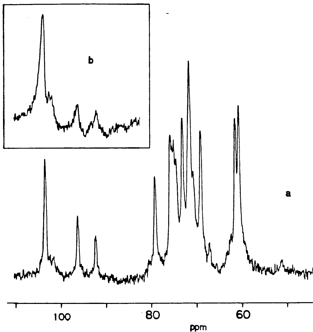
Fig. III-3. 100.6 MHz ^{13}\text{C} -nmr spectra of (a) [7] and (b) [6] (d.s. 0.9) obtained from [7] (a) after 5d dialysis; (contd.)
