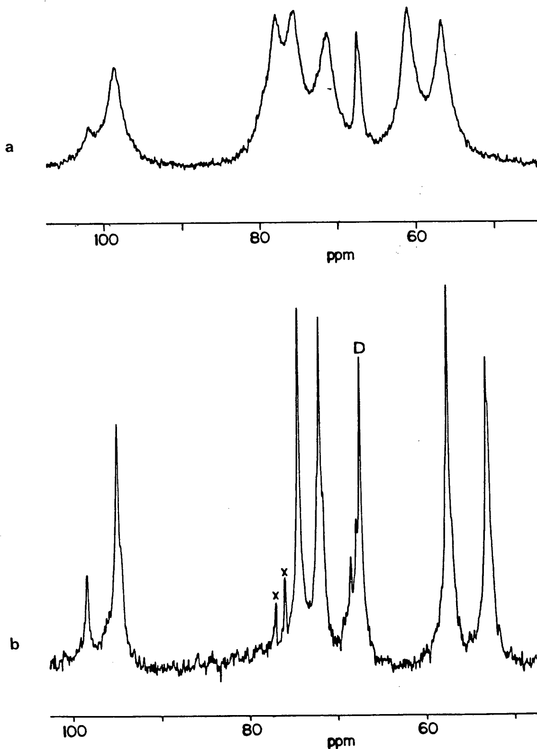
Fig. III-1. 100.6 MHz ^{13}\text{C} -nmr spectra of [1] (4% in \text{DOAc-d}_4/\text{D}_2\text{O} ) at 315K (a) at pD 4; (b) at pD 1.5; (sweep width 26,000, pulse width 13 \mu\text{sec} , delay 0.1 sec, 50 000 scans).
