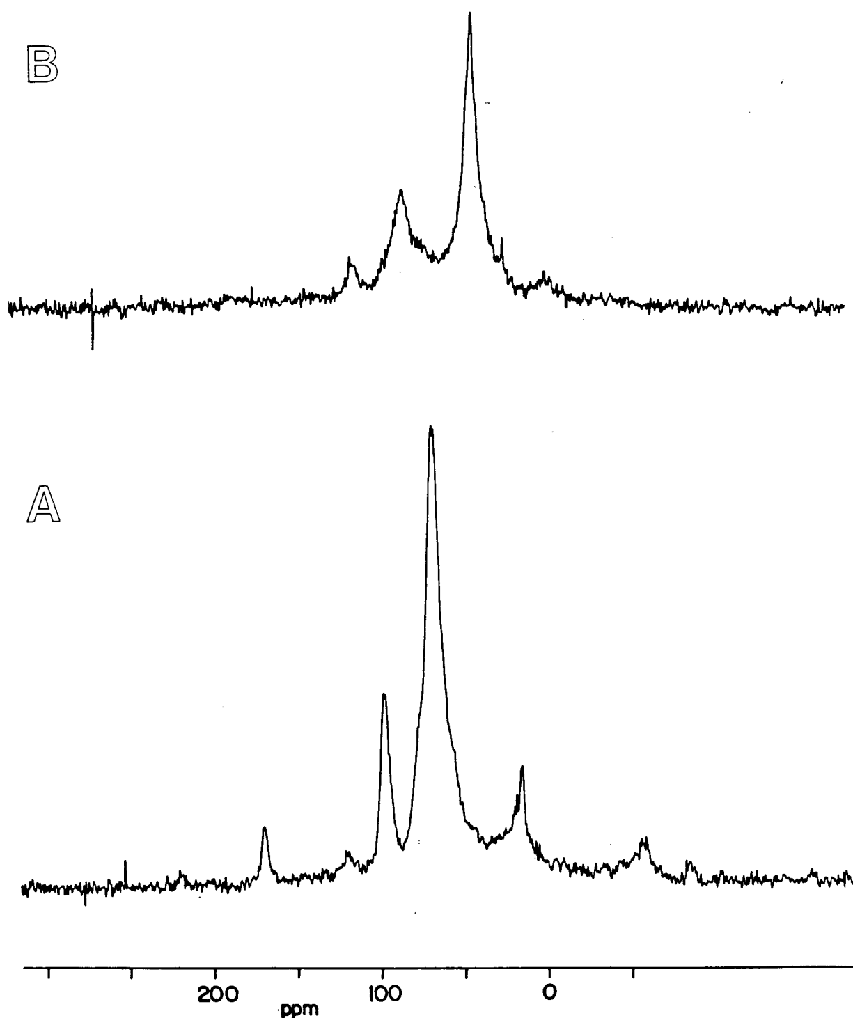
Fig. A-2. ^{13}\text{C} -MAS-CP nmr spectra of (A) xanthan gum (unpurified Keltrol), 10,000 scans, 2 s repetition, 0.5 ms contact time, 2 KHz spinning 10 G ^1\text{H} decoupling; (B) octadecyl xanthan amide, 100 mg sample, same conditions. Spectra were obtained on a Bruker CXP-200 spectrometer ( by Dr. S.Ganapathy).
