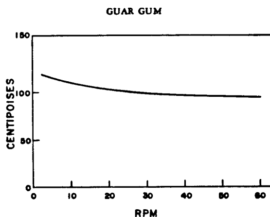
Fig. IV-9. Rheogram of a 0.3% food-grade guar gum solution at 25°C (from ref. 29).
