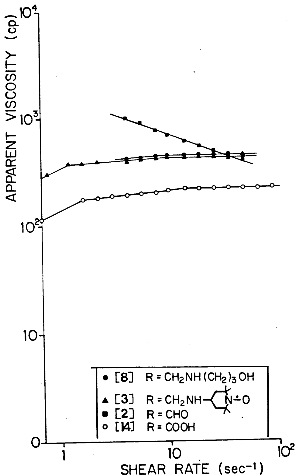
Fig. IV-8. Logarithmic plot of apparent viscosities of guaran derivatives versus shear stress.
