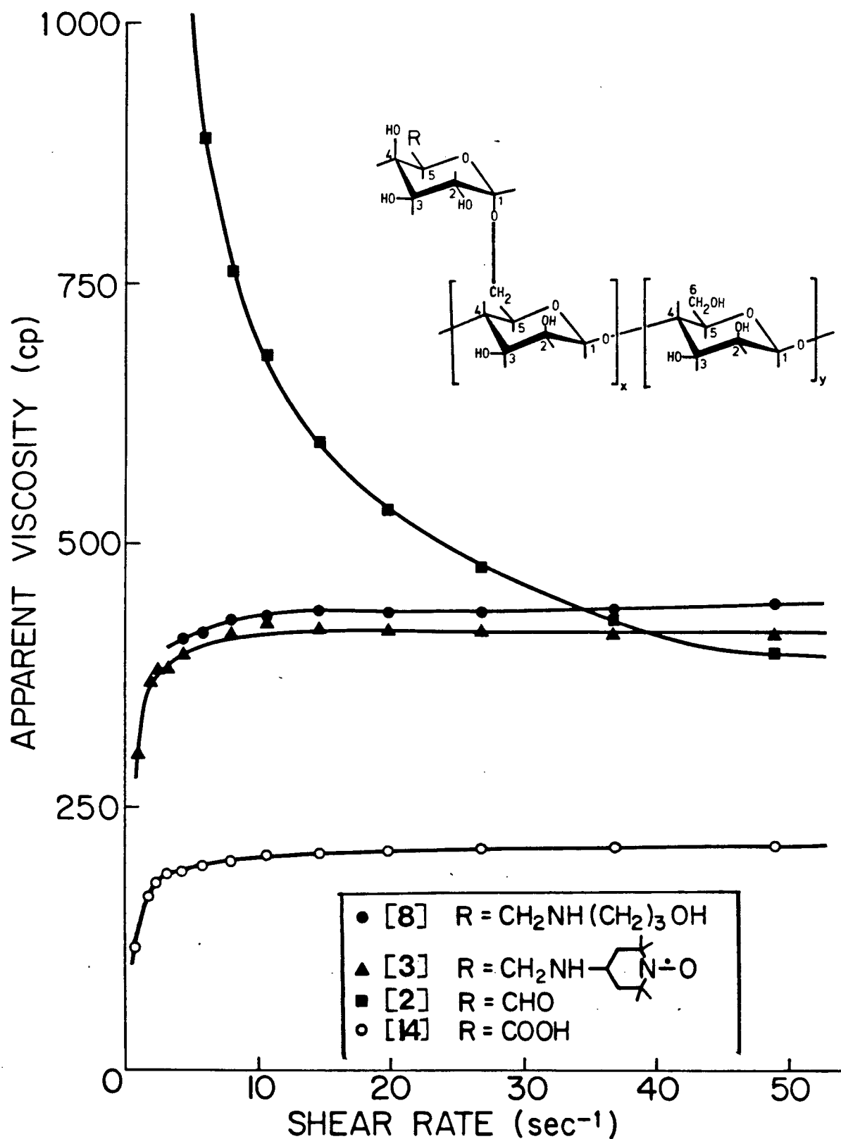
Fig. IV-7. Apparent viscosities of 1% aqueous solutions of guaran derivatives as a function of shear stress.
