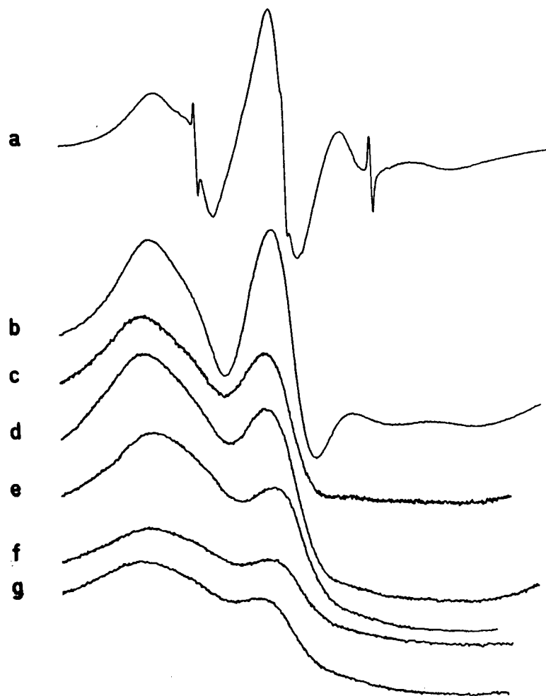
Fig. III-11. ESR spectra of [30] (left) and [29] (right) in the presence of Ni(II); Ni(II) concentrations were (mM): [30] (a) 0, (b) 1.12, (c) 2.23, (d) 3.35, (e) 5.59, (f) 16.76, (g) 25.69; [29] (a) 0, (b) 2.23, (c) 3.35, (d) 4.47.
