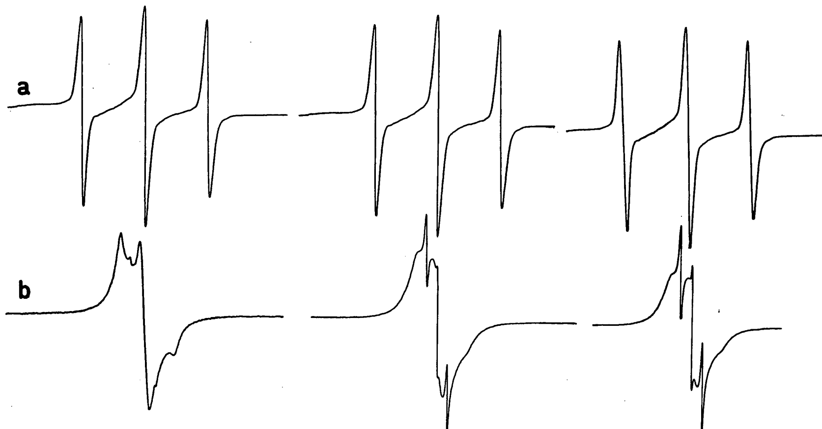
Fig. II-11. ESR spectra of [31] derived from dialdehyde cellulose samples ([30]) with d.o. 0.05 (left), 0.19 (centre), 0.34 (right), respectively; (a) aqueous suspension; (b) solid; (298K)
