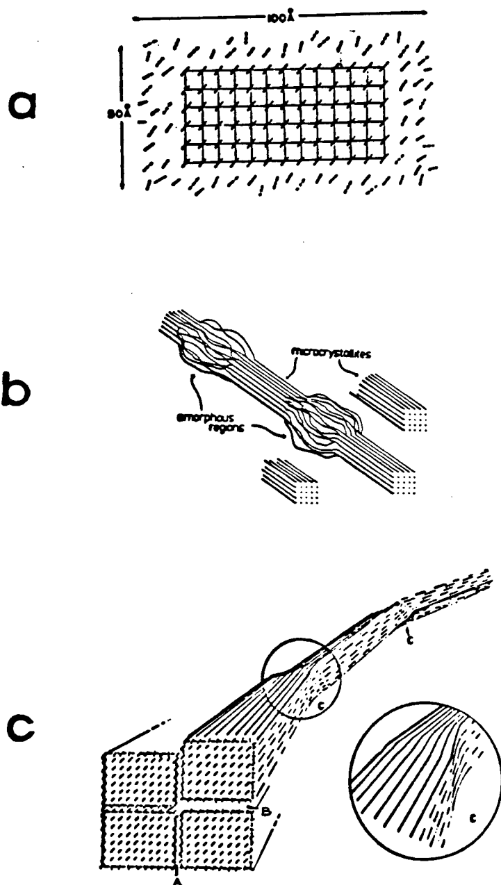
Fig. I-4. Proposed structures for the cellulose microfibril: (a) cross-section of fibril; order increases towards a central core (from ref. 18); (b) amorphous regions and microfibrillites within a single microfibril; (c) model incorporating elements of (a) and (b), three surface types are shown (A,B,C,).
