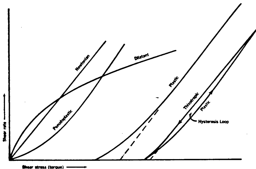
Fig. I-10. Rheological phenotypes (from ref. 49).
