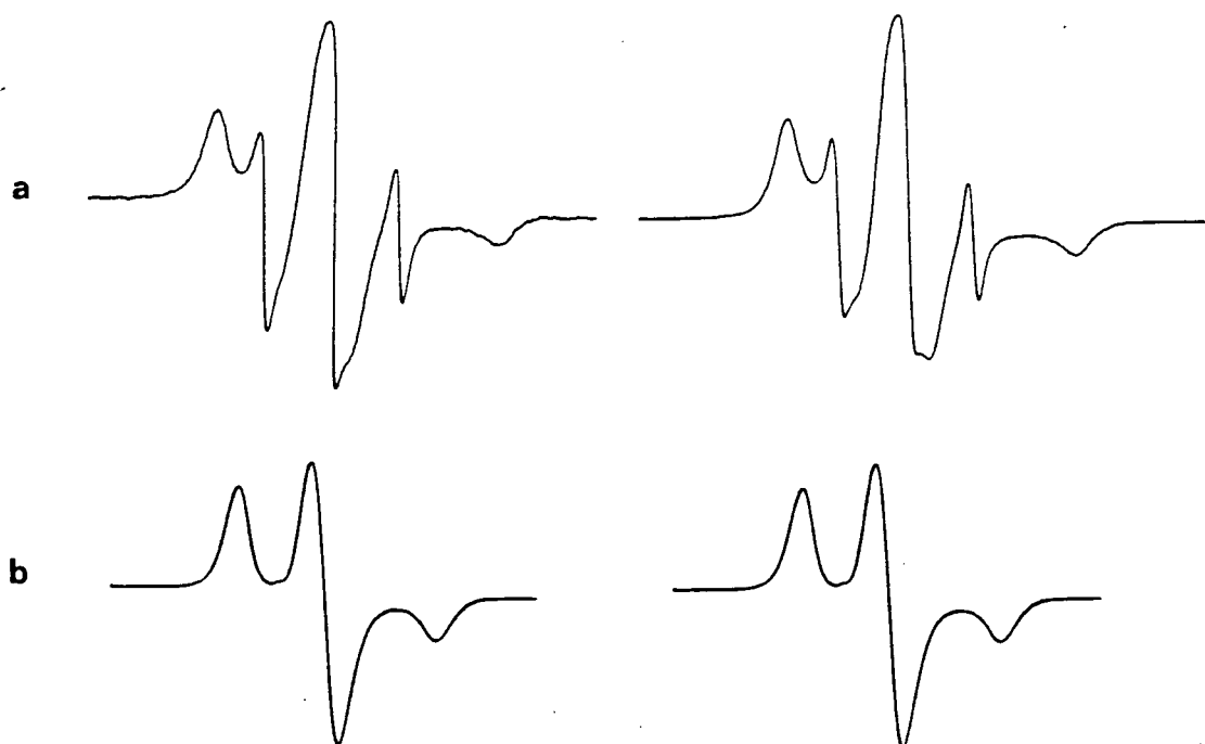
Fig. IV-11. ESR spectra of [21] (left) and [22] (right) (a) solid (at 298K), (b) frozen at 77K.
