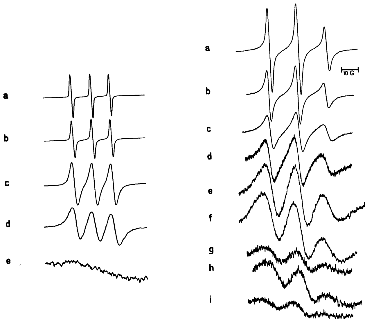
Fig. III-8. ESR spectra of [33] (left) and [35] (right) in the presence of Ni(II); Ni(II) concentrations were (mM): [33] (a) 0, (b) 0.12, (c) 0.23, (d) 0.45, (e) 1.12; [35] (a) 0, (b) 0.22, (c) 0.45, (d) 2.90, (e) 5.14, (f) 9.61, (g) 11.84, (h) 20.2, (i) 30.0.
