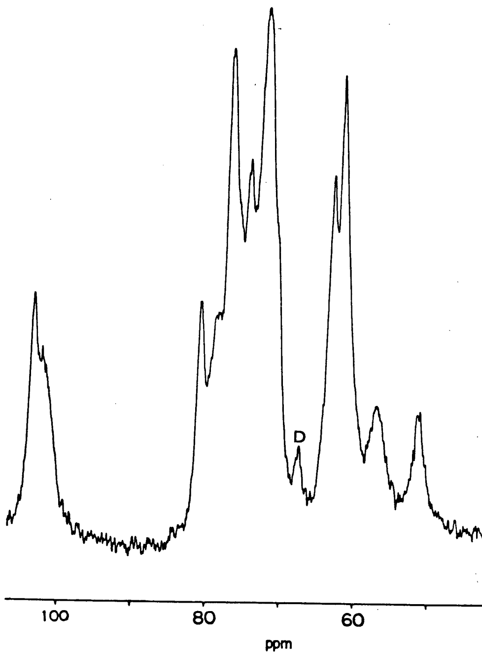
Fig. III-2. 100.6 MHz ^{13}\text{C} -nmr spectrum of [5] in \text{D}_2\text{O} (5%) at 315K; ( same conditions as for [1], 81 000 scans).
