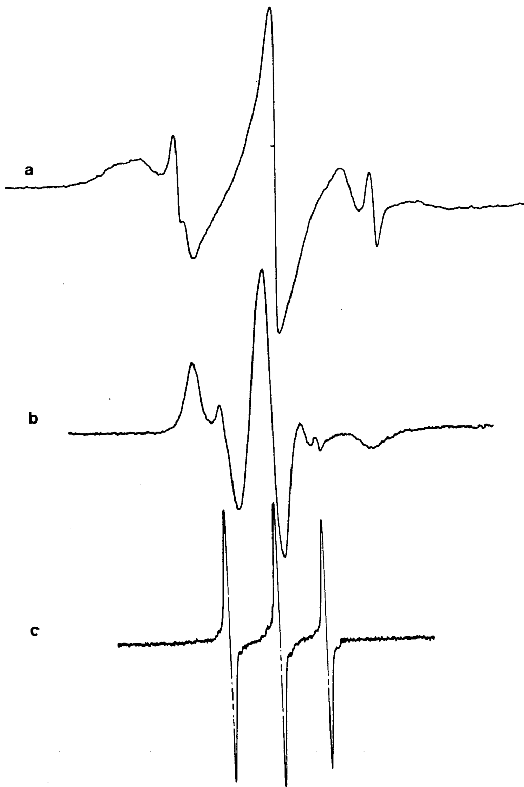
Fig. III-6. ESR spectra of [31] (a) gel in water, (b) gel in methanol, (c) gel (b) transferred into water (after 2 weeks equilibration); (at 298K).
