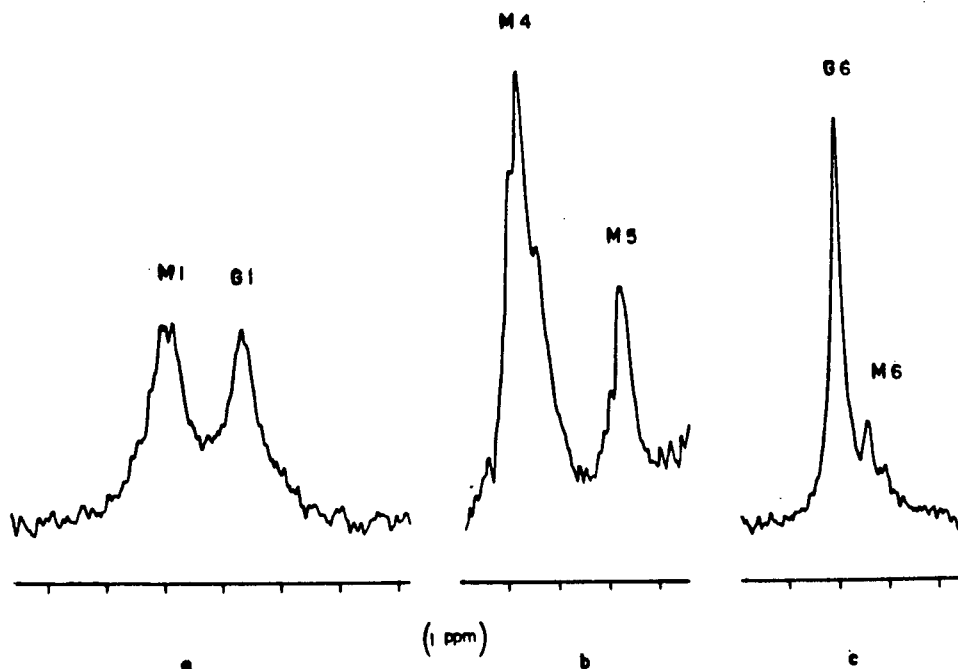
Fig. IV-6. ^{13}\text{C} -spectral region of (a) C1, (b) C4, C5, (c) C6 for [1].
