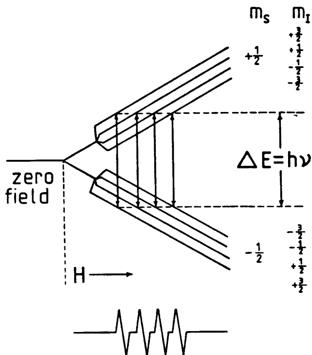
Fig. I-20. Spin state energy level diagram for a copper (II) nucleus in a magnetic field.
