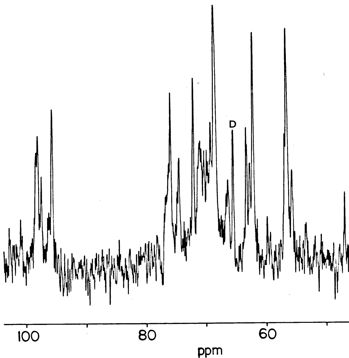
Fig. A-1. 100.6 MHz ^{13}\text{C} -nmr spectrum of xanthan gum (5%) in \text{D}_2\text{O} at 338K; (sweep width 26,000 Hz, 25,000 scans).
