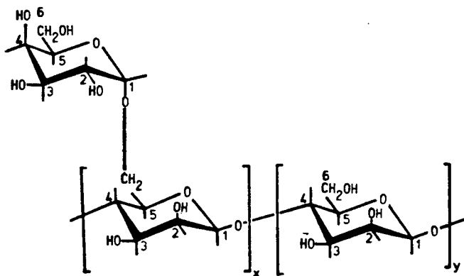
Fig. I-5. Composition of guaran ( x/y = 1.8 ) and locust bean gum ( x/y = 4.3 ) used in this study.
