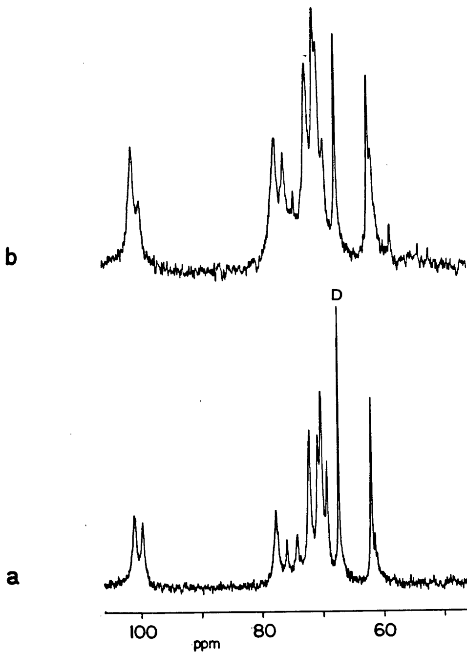
Fig. IV-5. 100.6 MHz ^{13}\text{C} -nmr spectra of (a) [1] and (b) [5] in \text{D}_2\text{O} ; (sweep width 23,000 Hz, pulse width 14 \mu\text{s} , delay 0.1 s, 50,000 scans).
