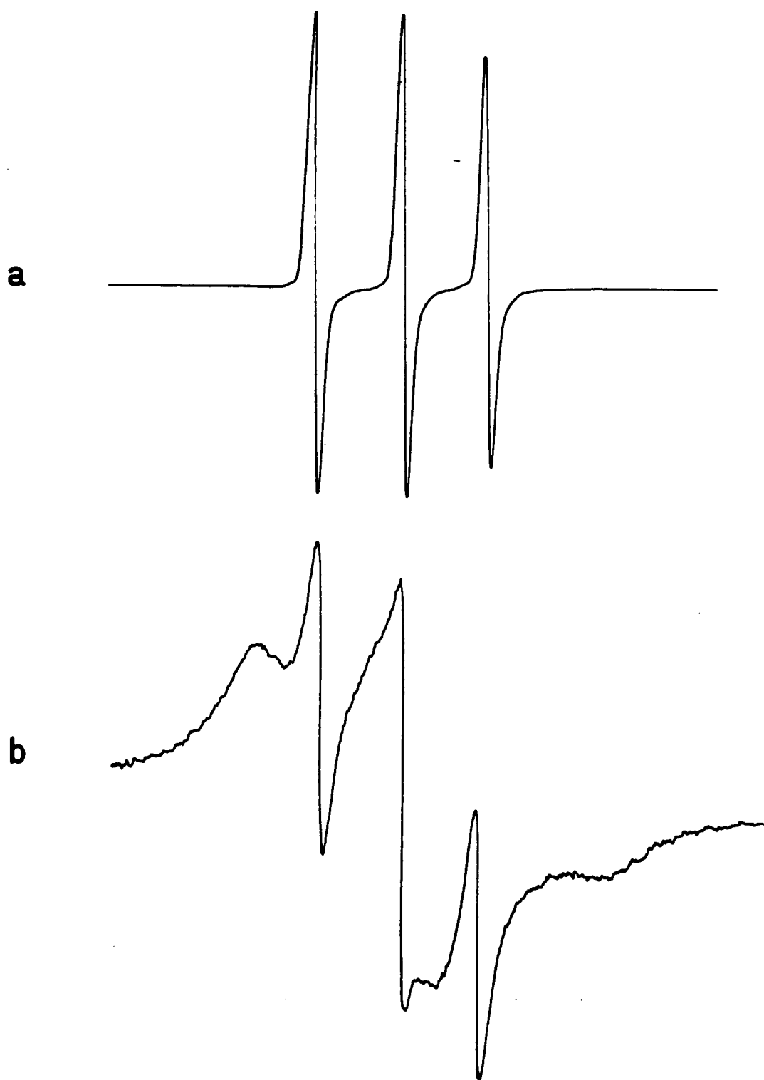
Fig. II-1. ESR spectra of [10] (a) in aqueous solution; (b) solid; (at 298 K).
