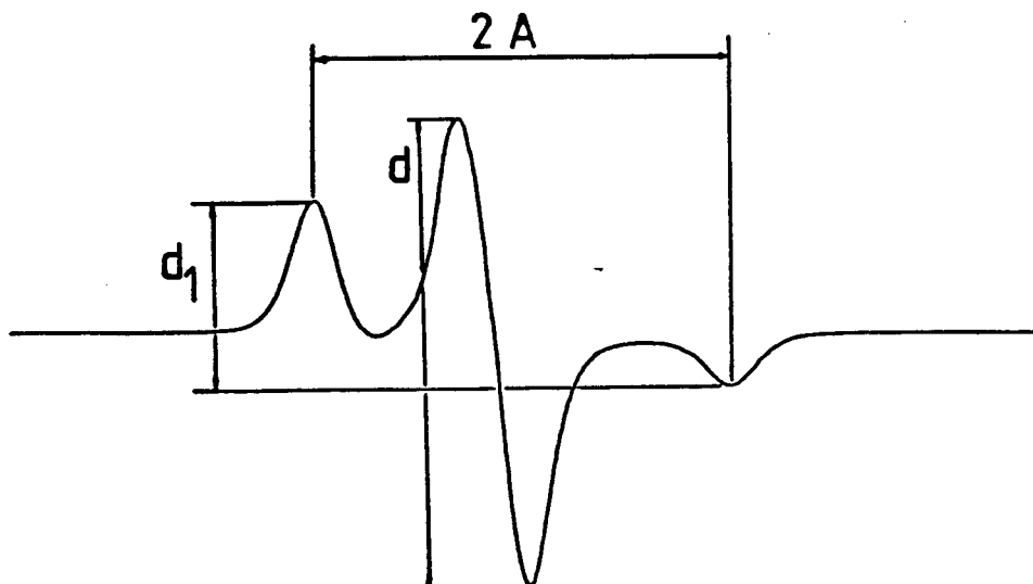
Fig. I-19. Powder spectrum showing the heights d_1 and d and the splitting 2A .
