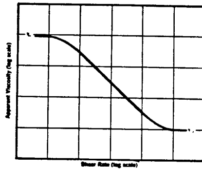
Fig. I-11. Logarithmic plot of apparent viscosity versus shear rate for a pseudoplastic fluid (from ref. 48).
