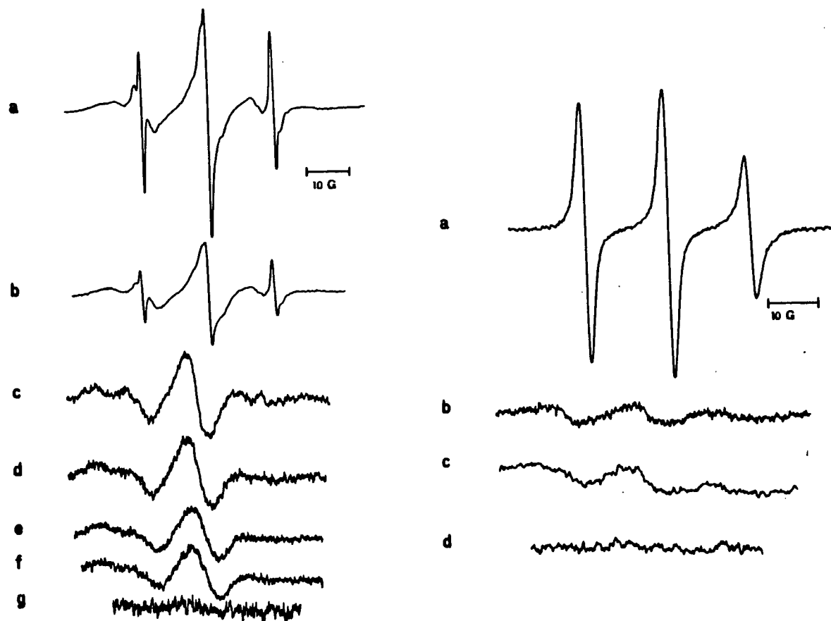
Fig. III-10. ESR spectra of [31] (left) and [34] (right) in the presence of Ni(II); Ni(II) concentrations were (mM): [31] (a) 0, (b) 2.23, (c) 4.47, (d) 6.70, (e) 8.94, (f) 13.40, (g) 31.28; [34] (a) 0, (b) 2.23, (c) 4.47, (d) 6.70.
