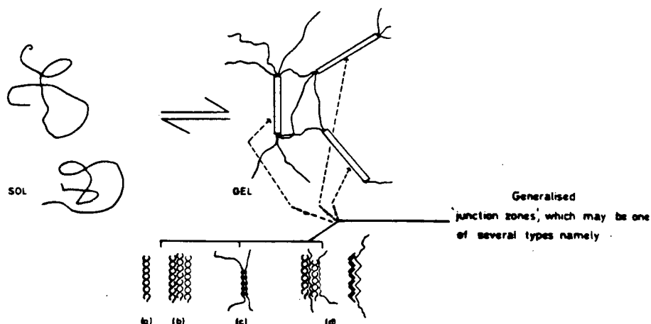
Fig. I-13. Generalized scheme for gelling of polysaccharides (from ref. 1).
