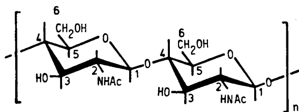
Fig. I-7. Structure of chitin.
