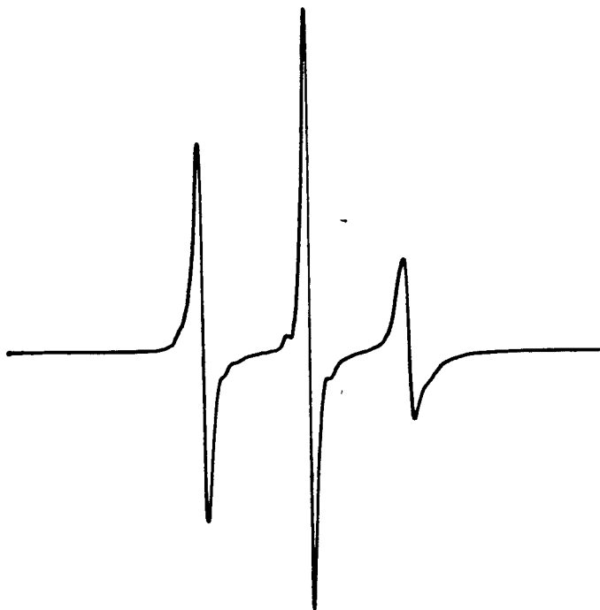
Fig. II-7. Esr spectrum of [21] in aqueous solution (at 298K).
