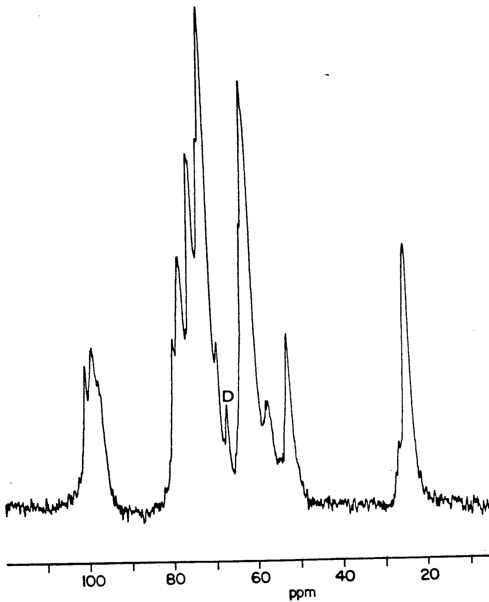
Fig. III-3. (continued) (c) ^{13}\text{C} -nmr of [6] ( d.s. 0.25); at 315K in \text{D}_2\text{O} .
