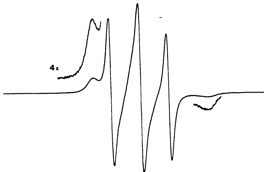
Fig. II-10. Esr spectrum of solid [27] under methanol (at 298K).
