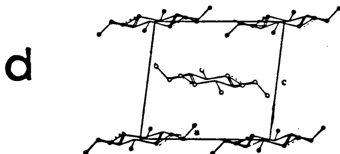
Fig. I-3. Structure of cellulose: (a) sequence; (b) chains resemble a flat ribbon; (c), (d) proposed chain packing
