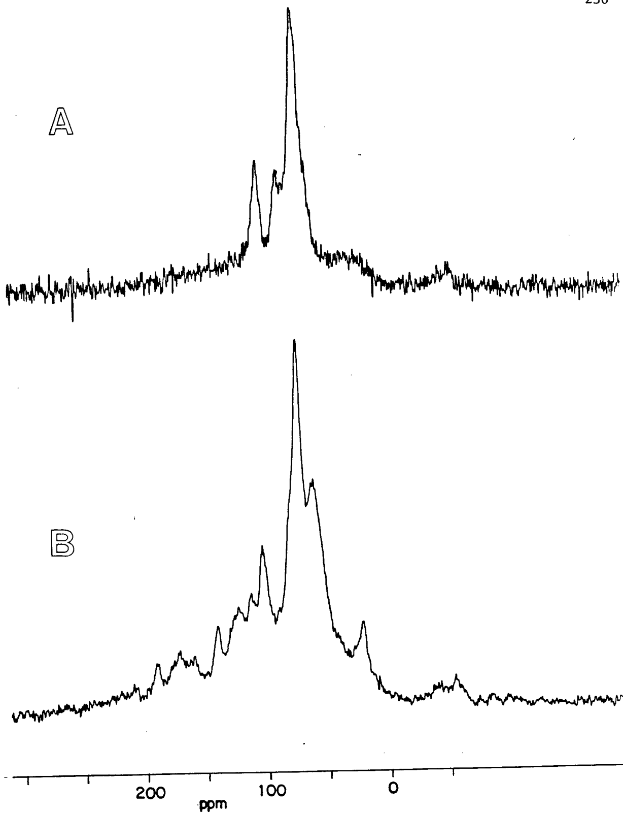
Fig. A-3. ^{13}\text{C} -MAS-CP nmr spectra of (A) cellulose (Whatman CF11), 10,000 scans, 2 s repetition, 0.5 ms contact time, 2 KHz spinning, 10 G ^1\text{H} decoupling; (B) [N-(3-fluoro)-benzyl] chitosan, 20,000 scans, same conditions.
