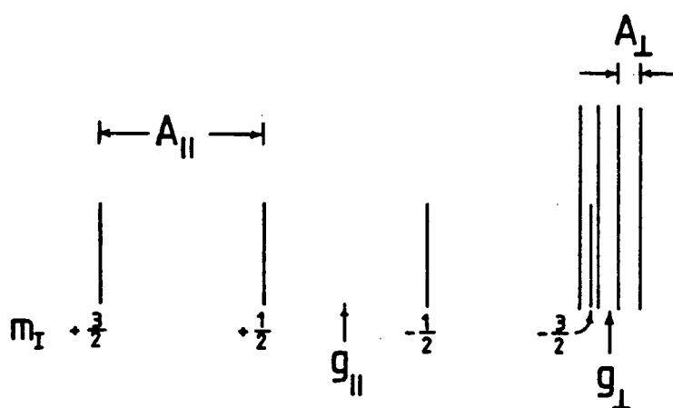
Fig. I-21. Scheme of copper (II) esr spectrum showing both g_{||} and g_{\perp} components.
