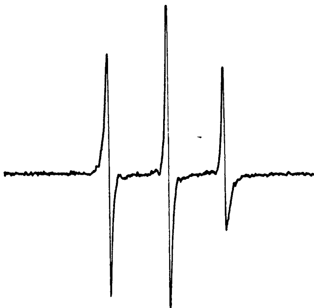
Fig. II-14. Esr spectrum of [40] in aqueous solution (298K).
