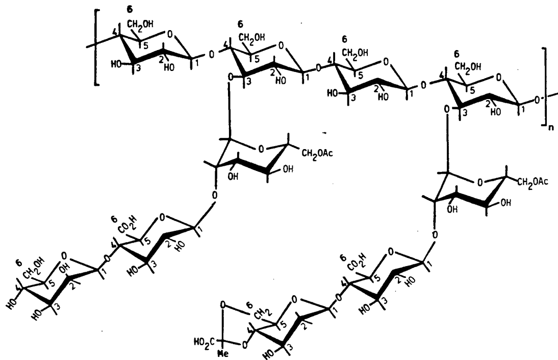
Fig. I-2. Structure of xanthan gum.
