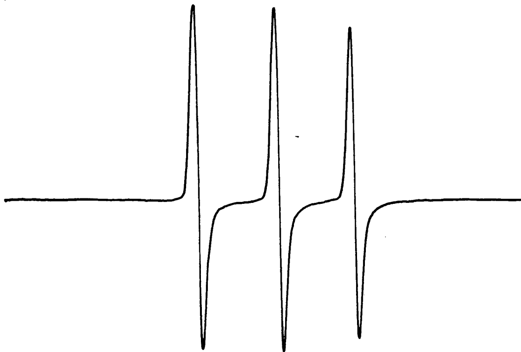
Fig. II-9. Esr spectrum of [26] in aqueous solution (at 298K).
