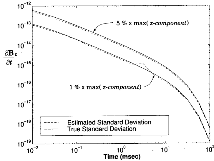
Figure 5.6: Noise model recovered in two synthetic test cases. In the first case, the standard deviation of the assigned noise was set to be a 5% of the maximum value of the Z -component of the data of that time channel. In the second case the standard deviation of the assigned noise was set to 1% of the maximum. Solid lines represent the noise assigned in each time channel, and dashed lines represent the estimated noise by inverting each time channel for a pair of dipoles. The technique was successful in recovering the noise.
