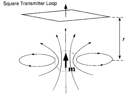
Figure 3.11: Approximating the response of an arbitrary compact object by that of the sphere. Directly above a sphere, the response looks like a single decay dipole located at the sphere center and located at a distance r from the square transmitter loop.
