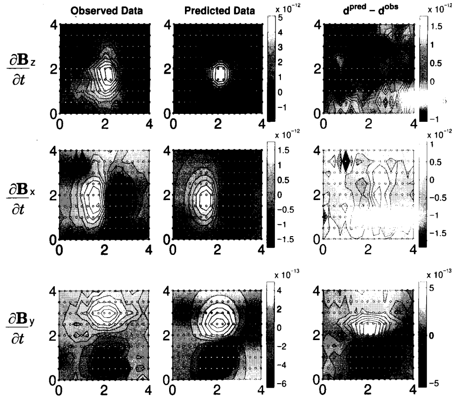
Figure 5.7: Inversion of t = 0.036 \text{ msec} time channel \partial \mathbf{B} / \partial t data acquired over a 105 mm UXO buried at the York University Environmental Test Site.
