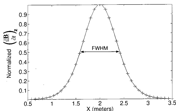
Figure 3.8: Definition of the “Full Width at Half Maximum” (FWHM). The width of a profile provides an estimate of the depth. The FWHM value in this example is 0.82 m. Extra care must be taken when there are multiple peaks.
