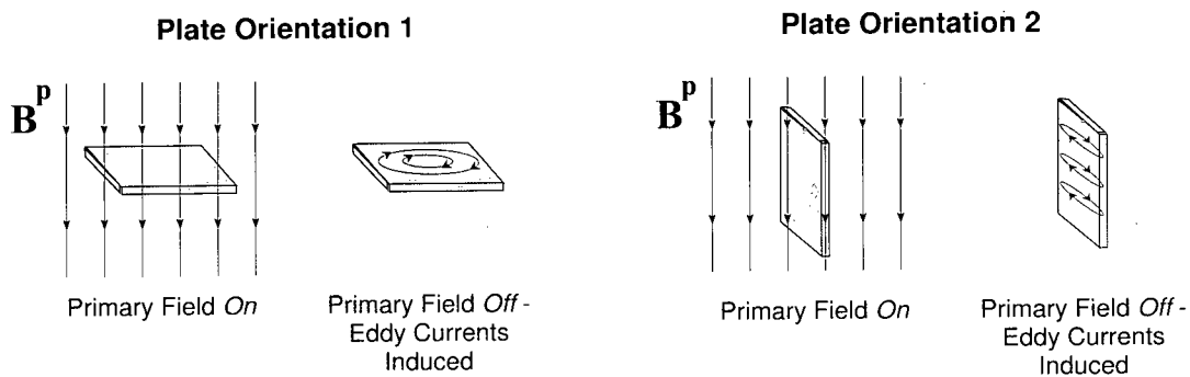
Figure 4.3: Eddy current induction in a non-permeable plate. When the direction of the primary field B^p is normal to the plane of the plate there is a maximum coupling between the field and the plate. The field and plate are minimally coupled when the primary field is parallel to the plane of the plate.
