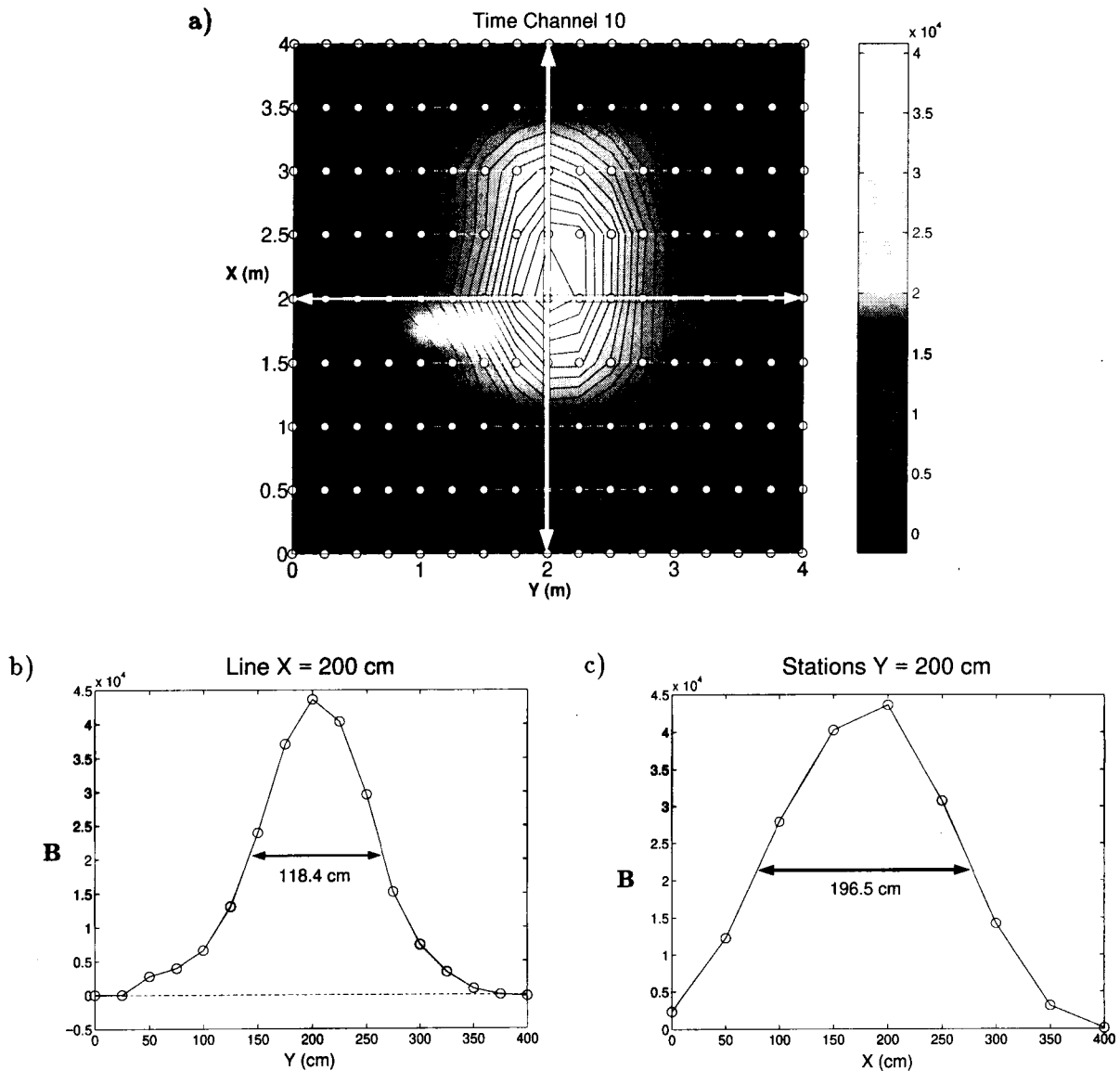
Figure 5.12: Determining the depth of the buried UXO. Panel (a) contains a plot of the vertical component of the \mathbf{B} -field measured during the tenth time channel. The two white lines indicates where profiles of the signal have been taken for depth estimation. Panel (b) contains a profile taken along the Line X = 200 cm. The depth estimate (from the ground surface to the center of the target) using this profile is 76.4 cm. Panel (c) contains a profile taken perpendicular to the lines on stations Y = 200 cm. The depth estimate using this profile is 152.5 cm.
