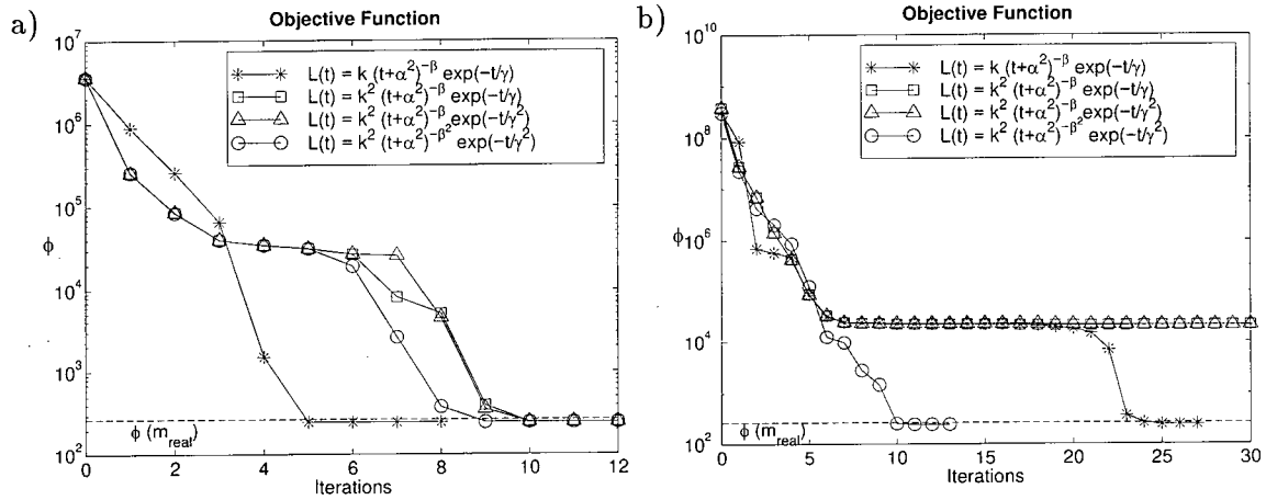
Figure 3.23: Convergence behaviour when using various variable transformations. (a) When using the standard starting guess, each of the different transformations on the model parameters converge to the correct parameters. (b) When the starting guess is taken further away from the solution (using equation 3.48, transformations to a more non-linear objective function lead to a cases where the inversion doesn't converge to the right answer.
