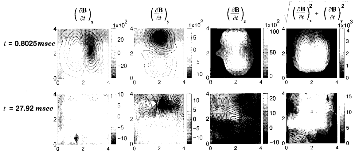
Figure 3.1: The \partial \mathbf{B}/\partial t measurement taken over a 105 mm shell. At earlier times the signal has the appearance of a dipole field. With later times the signal from the UXO is dominated by the noise.
