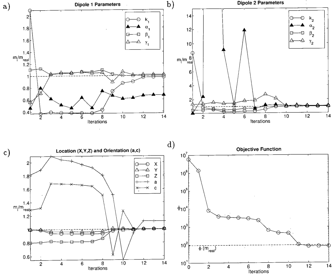
Figure 3.21: Convergence results when maxstep = 10 \times \|\mathbf{m}_{typ}\| . The correct model parameters are recovered by the inversion. Panel (d) plots the values of the objective function with each iteration. The inversion achieved a data misfit that is less than the objective function to the level that would be achieved if the real model parameters were recovered. This indicates that some of the noise is being fit.
