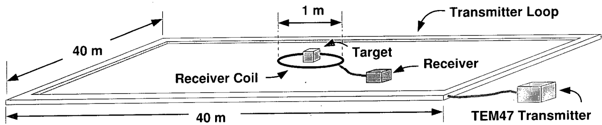
Figure 4.1: Geonics Laboratory Setup
