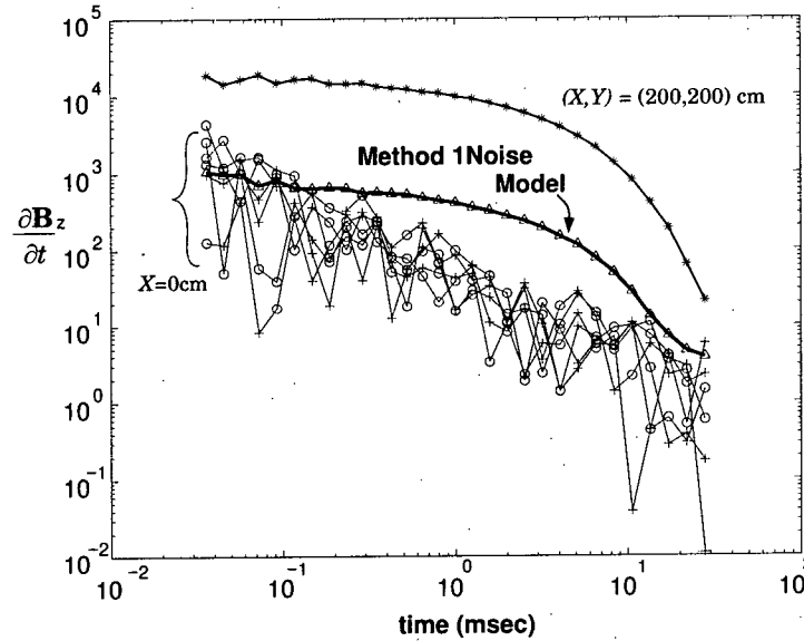
Figure 5.8: Noise model recovered for the field data by fitting a pair of dipoles to each time channel. The recovered noise model is plotted, along with the Z -component \partial \mathbf{B} / \partial t response measured directly above the UXO ( (X, Y) = (200, 200) cm), and several (noisy) decay curves measured along the X = 0 cm line.
