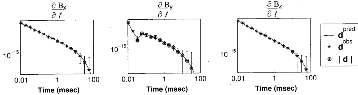
Figure 3.3: The synthetic \partial \mathbf{B} / \partial t response curves for a 75 mm anti tank mortar buried 58 cm beneath the surface. The circled data points indicate that the absolute value of the data point has been plotted.
