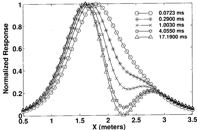
Figure 3.7: Estimating the depth and location of a thick steel rod with c = 70 at various times. The real "Location on Profile" is actually 2 m, and the real depth is 1 m.
