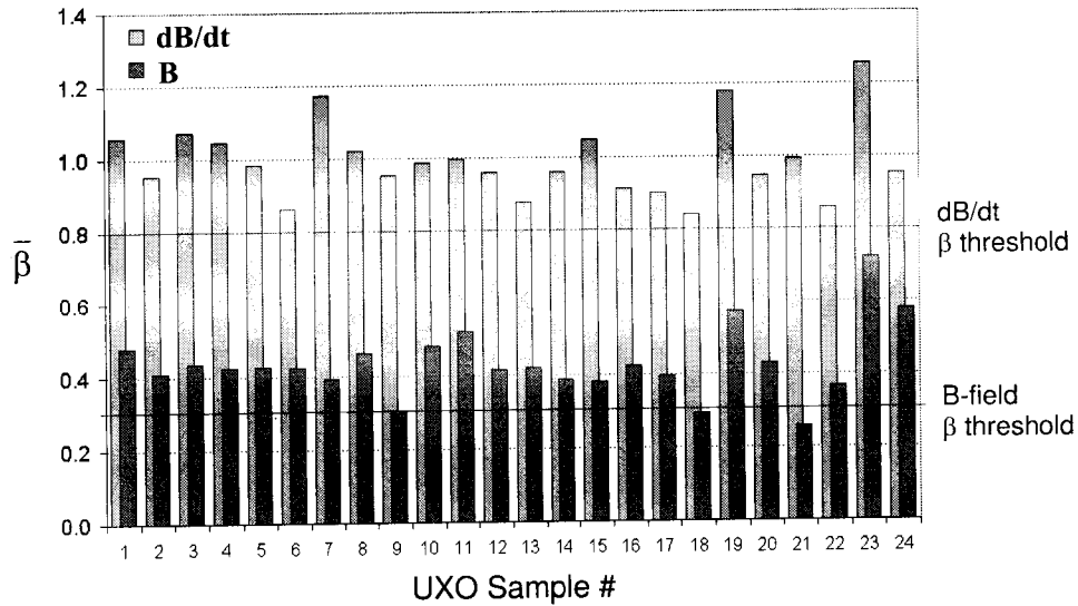
Figure 4.14: \bar{\beta} averages for UXO. When fitting the \partial \mathbf{B} / \partial t response of a UXO with the parameterization, the average of the recovered \beta 's ( (\beta_1 + \beta_2) / 2 = \bar{\beta} ) is greater than 0.8. When fitting the \mathbf{B} -field response of a UXO with the parameterization, the average of the recovered \beta 's is greater than 0.3 (with the exception of UXO sample 21).
