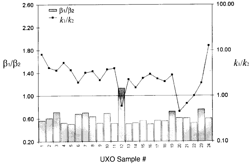
Figure 4.15: k_1/k_2 and \beta_1/\beta_2 ratios when fitting to derivative of field \partial \mathbf{B}/\partial t . The \beta_1/\beta_2 ratio is plotted with bars, and the line is the plotted k_1/k_2 ratio for each of the UXO. Recall that for a permeable rod-like prisms that k_1/k_2 > 1 and \beta_1/\beta_2 < 1 .
