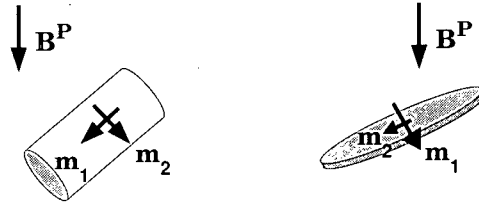
Figure 2.13: Representation of the fields generated by induced fields in a metallic target as a pair of orthogonal dipoles. Both dipoles are located at the center of the target, with Dipole 1 being parallel to the axis of symmetry of the target and Dipole 2 being perpendicular to the axis of symmetry and in a plane defined by the primary field and Dipole 1. The moment of each dipole is proportional to the projection of the primary field onto a unit vector in the dipole direction.
