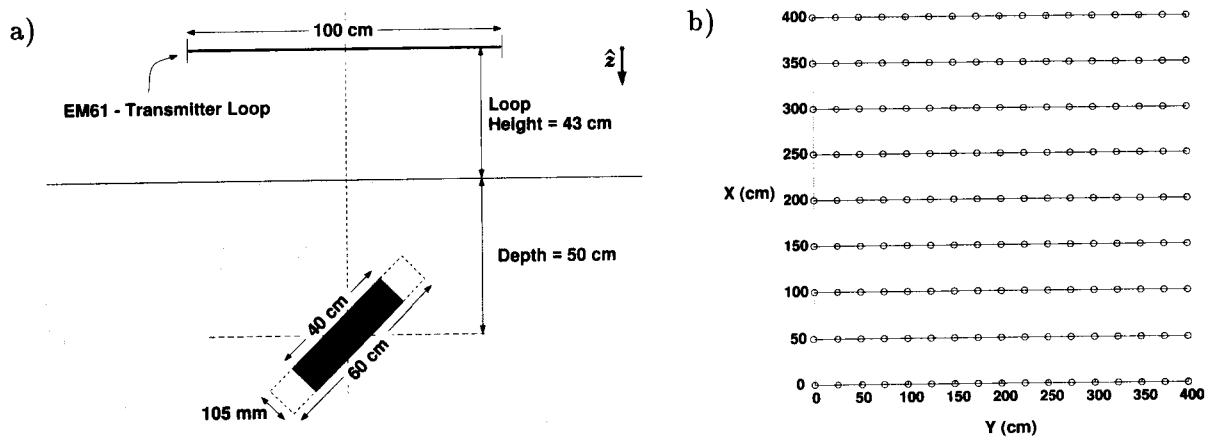
Figure 5.2: (a) The 105 mm shell buried as part of the York University Test Site was buried at a depth of 50 cm. The transmitter loop is mounted on a trailer, and therefore sits parallel to the ground at a height of 43 cm. (b) Line and station layout of the the field data survey grid. The component data were collected on 9 lines, with a line spacing of 50 cm. A total of 17 stations were spotted on the line, with a station separation of 25 cm. The coordinate system was set up such that the Z direction points into the ground.
