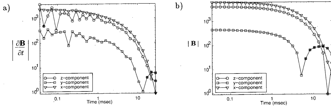
Figure 3.2: Decay of the response at (X, Y) = (1m, 1m) (a) The early time channels for the \partial \mathbf{B} / \partial t response is very noisy, and need not be fit too closely. (b) The process of integration smooths the response for \mathbf{B} .
