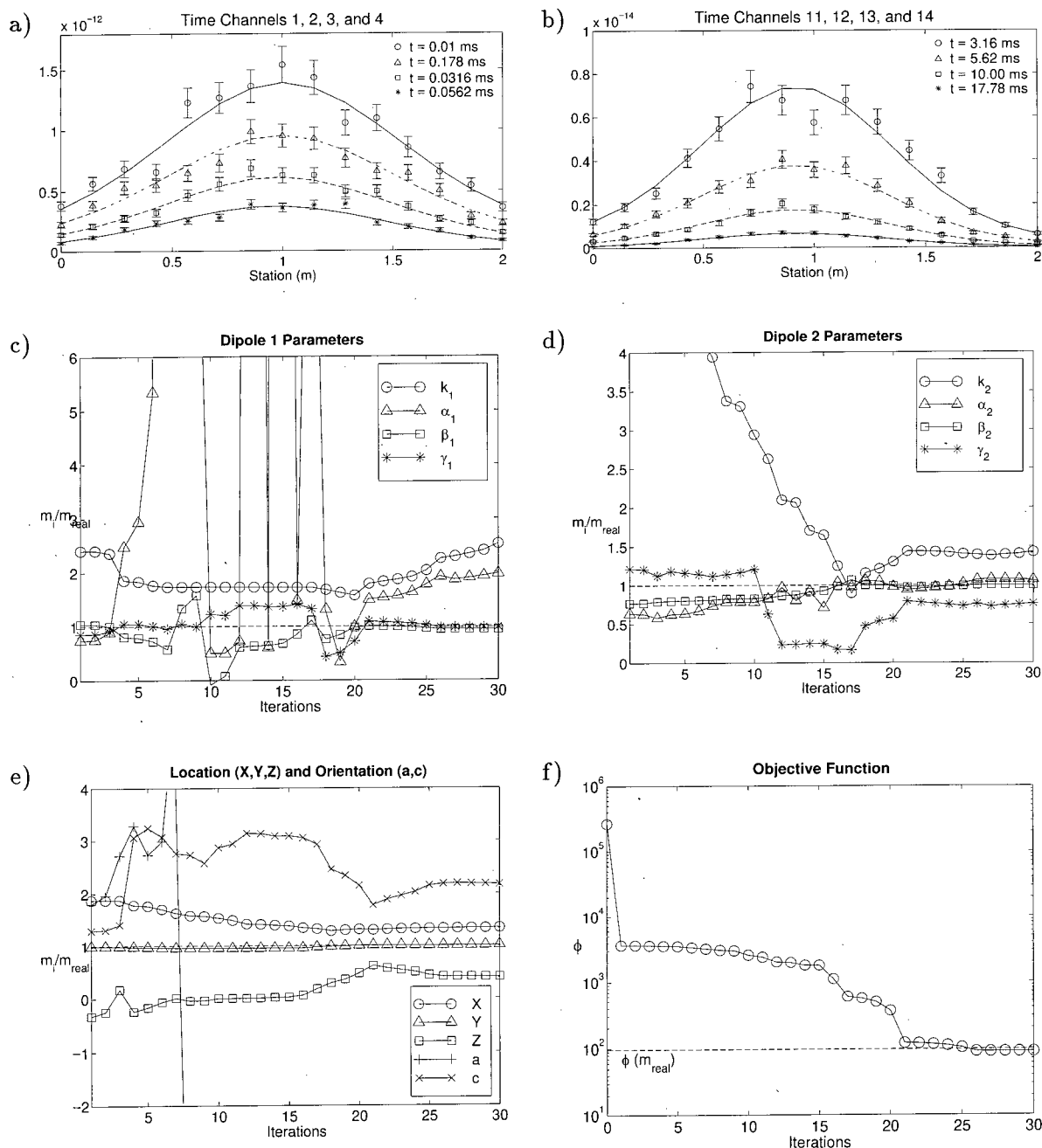
Figure 3.30: Results from inverting only the Z-component of the \partial \mathbf{B} / \partial t data of Line X=0m. Panels (a) and (b) include the observed and predicted data from both early and late times, indicating a good data fit in both cases. Panels (c), (d), and (e) include the model parameters as a function of iteration. It is clear that the inversion has been unable to successfully recover the correct model parameters even though the data has been well fit. Panel (f) shows that the final data misfit is lower than when the data misfit is calculated using the real model.
