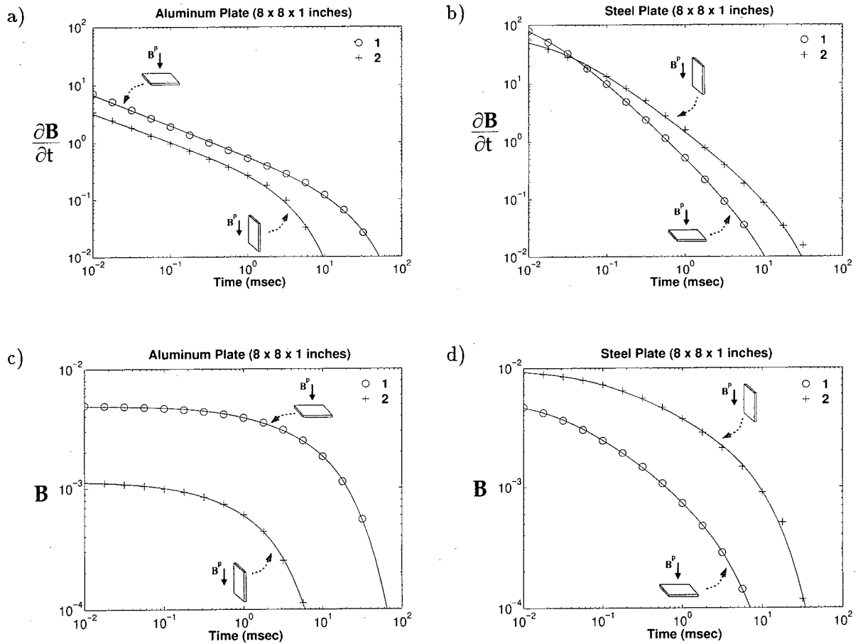
Figure 4.4: Time Decay curves for 8 \times 8 \times 1 inch steel and aluminum plates. Panels (a) and (b) contain the measured \partial\mathbf{B}/\partial t response. Panels (c) and (d) contain the \mathbf{B} -field response integrated from the measured \partial\mathbf{B}/\partial t response.
