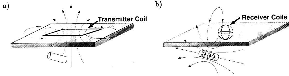
Figure 2.1: The induction of currents in a buried confined conductor. (a) Transmitter on-time. A transmitter, consisting of a square current-carrying coil, produces a primary magnetic field that illuminates the buried target. (b) Transmitter off-time. Once the transmitter current is terminated, the changing magnetic field induces currents in the buried conductive object. The induced currents produce a secondary field that is measured by receiver coils at the surface.
