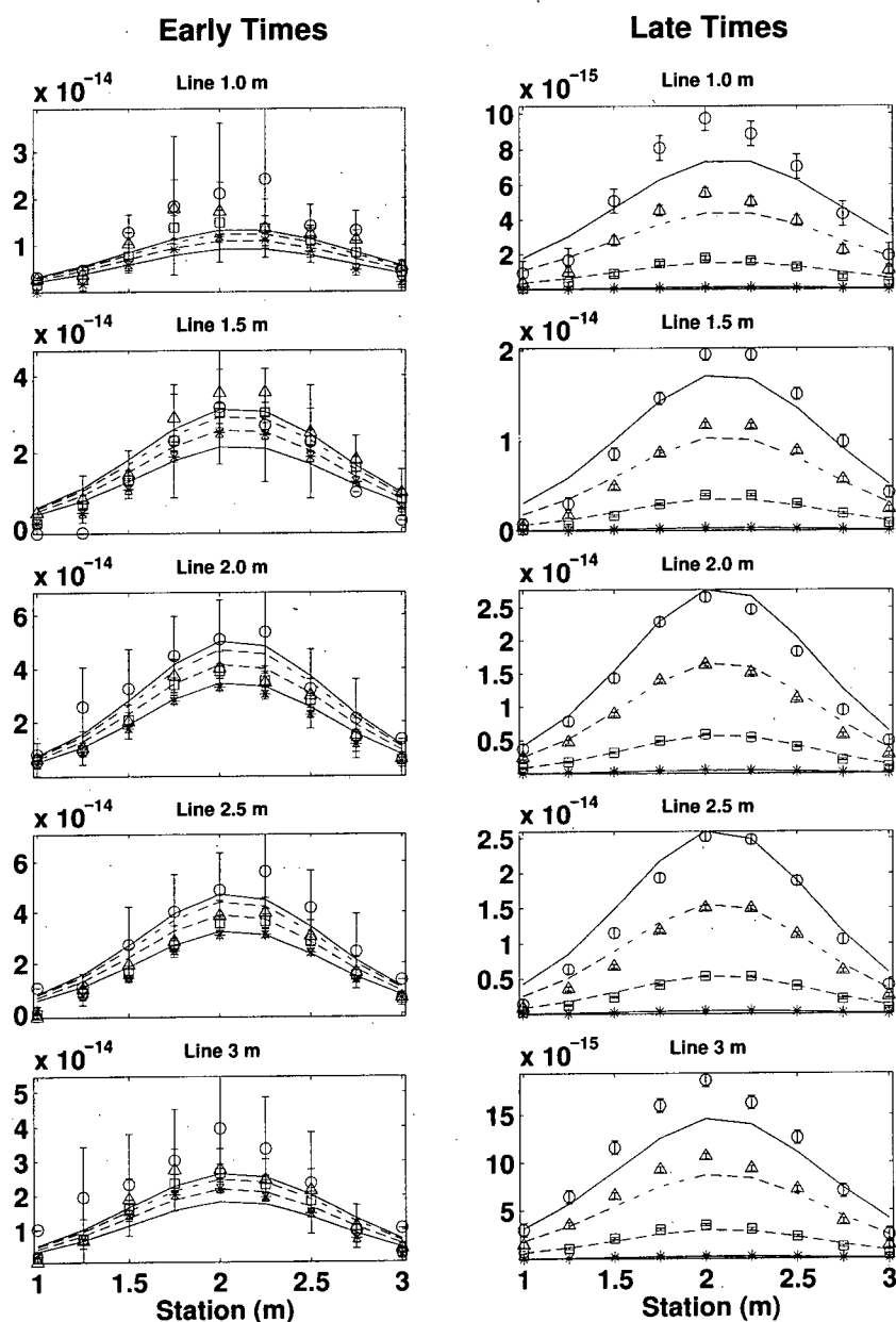
Figure 5.17: Observed and predicted data when inverting the Z -component of the \partial \mathbf{B} / \partial t field. The left column includes the data from some of the early time channels: t = 0.036 \text{ ms} (○), 0.092 \text{ ms} (△), 0.234 \text{ ms} (□), and 0.525 \text{ ms} (*). The right column of Figure 5.17 include the data from t = 1.003 \text{ ms} (○), 2.53 \text{ ms} (△), 6.54 \text{ ms} (□), and 17.2 \text{ ms} (*). The error bars represent the standard deviation of the error assigned to each data point. The predicted does not fit to within the errors specified by the error bars.
