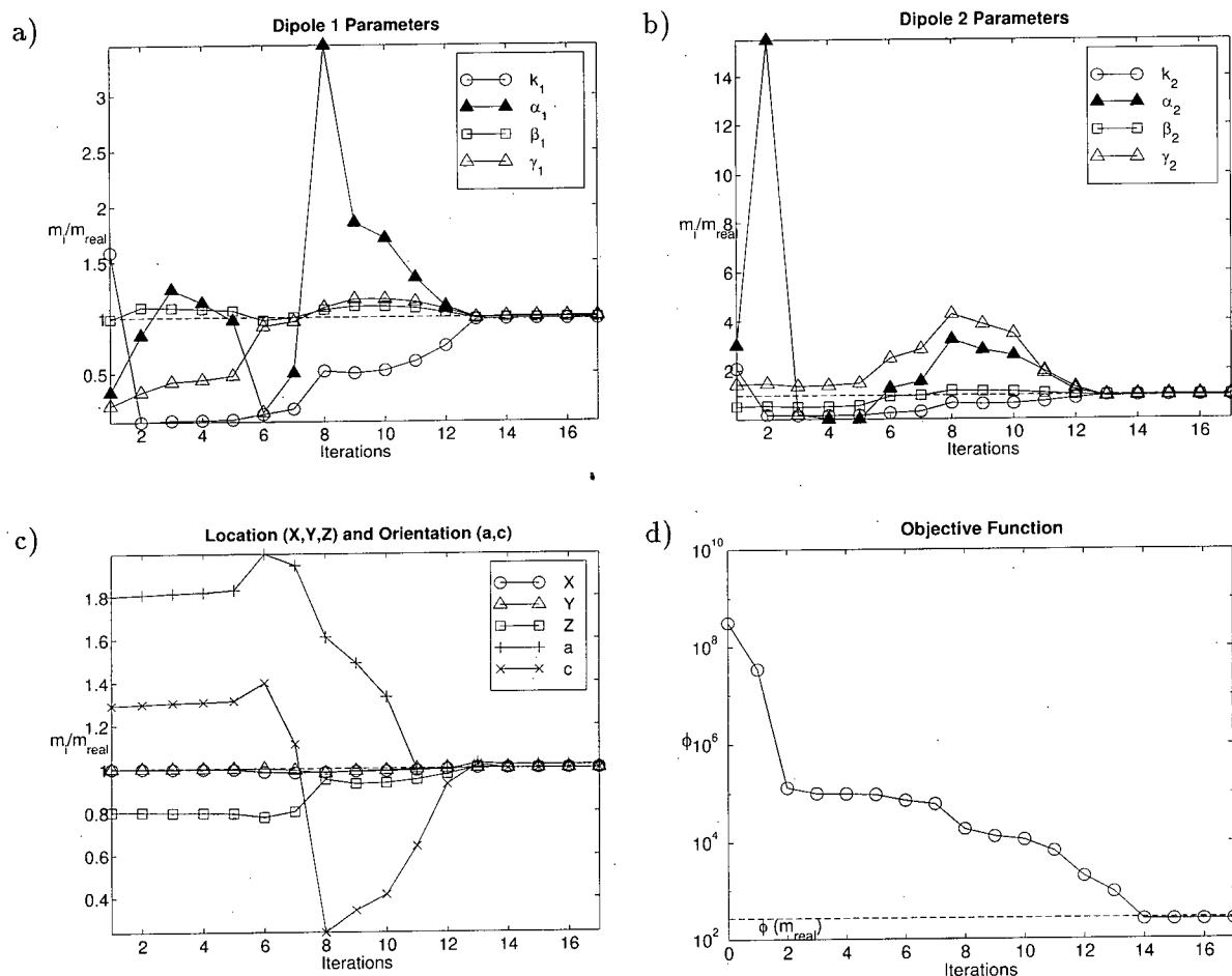
Figure 3.24: Convergence results when \kappa = 2 . Panels (a), (b), and (c) contain plots of the progress of the model parameters (scaled by the value of the real model parameter) as a function of iteration. The recovered parameters converge to the correct model parameters within 17 iterations. Panel (d) plots the values of the objective function with each iteration. The inversion achieved a final data misfit less than would be achieved when calculated with the true model.
