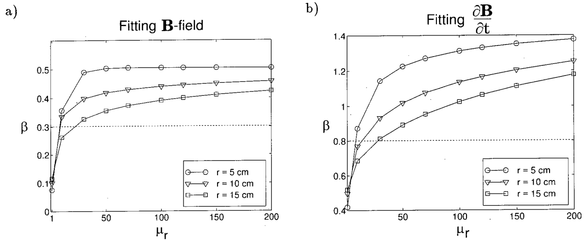
Figure 4.7: The behaviour of parameter \beta for various size spheres with varying permeability \mu . Panel (a) contains results of fitting the \mathbf{B} -field with the parameterization. Panel (b) contains results of fitting the \partial \mathbf{B} / \partial t with the parameterization. Each set of data is fit with the approximate forward model.
