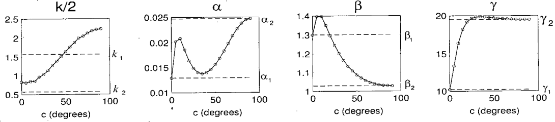
Figure 3.12: Results from fitting the Z-component of the response measured directly over steel rod ( 8 \times 1 \times 1 ).
