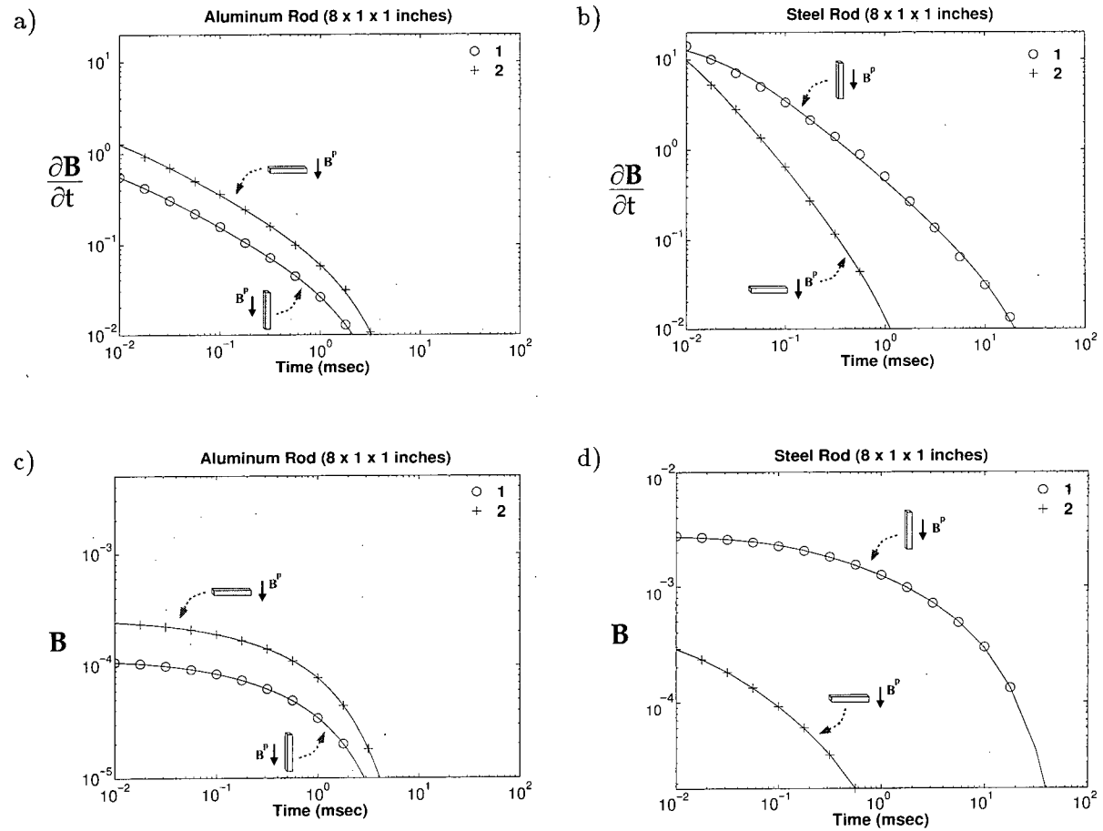
Figure 4.6: Time Decay curves for 8x1x1 inch steel and aluminum rods. Panels (a) and (b) contain the measured \partial \mathbf{B} / \partial t response. Panels (c) and (d) contain the \mathbf{B} -field response integrated from the measured \partial \mathbf{B} / \partial t response. Each set of data is fit with the approximate forward model.
