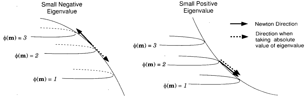
Figure 3.14: Small eigenvalues indicate either a ridge or a trough in the quadratic model of \phi . A small positive eigenvalue corresponds to a direction down a ridge. A small negative eigenvalue corresponds to a direction up a ridge. The direction can be reversed to point down the ridge by taking the absolute value of the eigenvalue as in equation 3.32 (After Bard, 1974).
