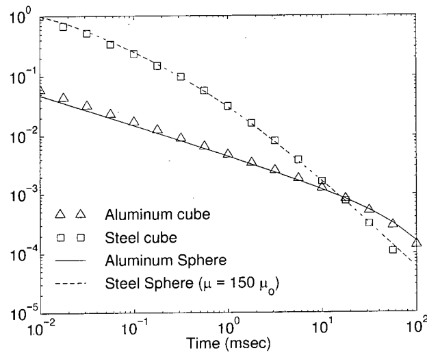
Figure 2.10: The responses of a metallic cube compared to a sphere of equal volume. The \partial \mathbf{B} / \partial t responses of the cubes were normalized by the measured value of the steel cube at t = 0.01 \text{ msec} . The responses of the spheres were normalized by the calculated value for a steel sphere at t = 0.01 \text{ msec} . Normalization was required to counter any extra gain in the signal during measurement.
