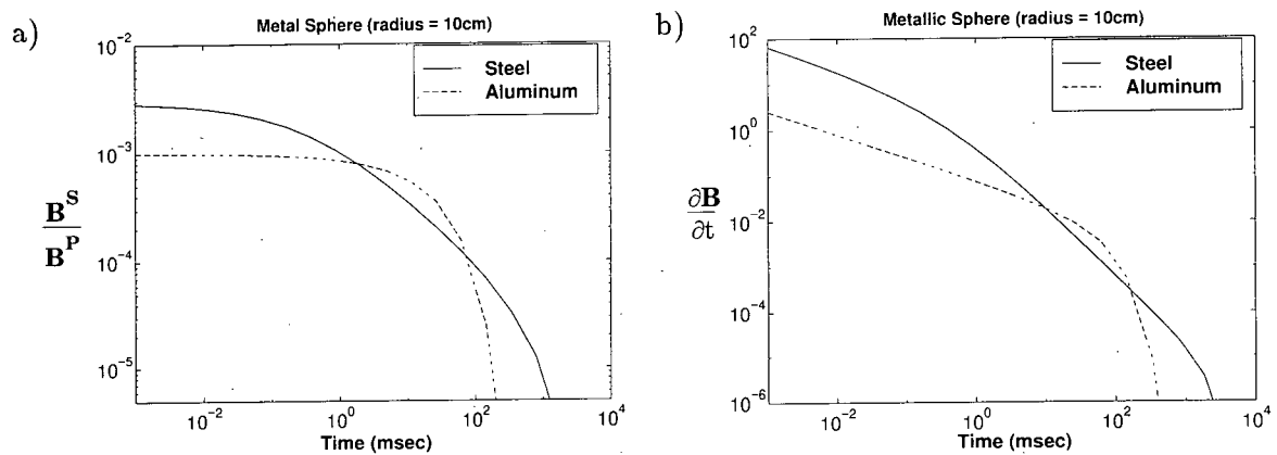
Figure 2.9: (a) The time decay behaviour of the magnetic flux density \mathbf{B} . The \mathbf{B} -field response is normalized by the strength of the primary field. (b) The time decay behaviour of the time derivative of the magnetic field \partial \mathbf{B} / \partial t .
