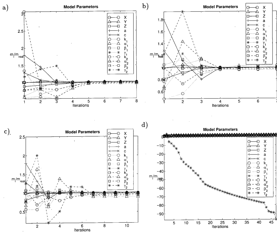
Figure 3.27: Using only a portion of the time channels. (a) All time channels are used. (b) Only odd time channels are used. (c) Time channels 1, 4, 7, 10, 13, and 16 are used. (d) Time channels 1, 5, 9, 13, and 17 are used.
