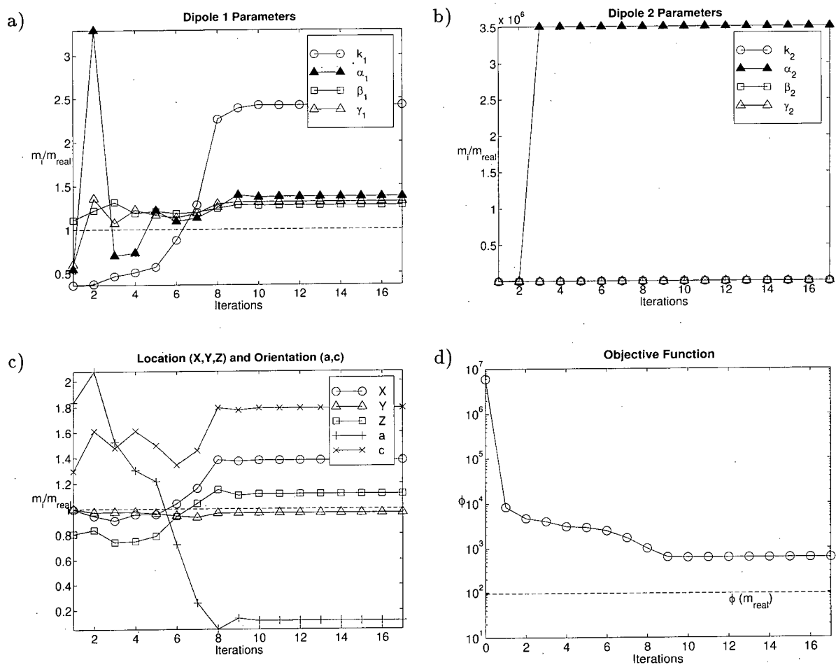
Figure 3.20: Convergence results when maxstep = 1000 \times \|\mathbf{m}_{typ}\| . The recovered parameters fail to converge to the correct model parameters. The recovery of \alpha_2 is particularly poor in this example. Panel (d) plots the values of the objective function with each iteration. The inversion was unable to reduce the objective function to the level that would be achieved if the real model parameters were recovered.
