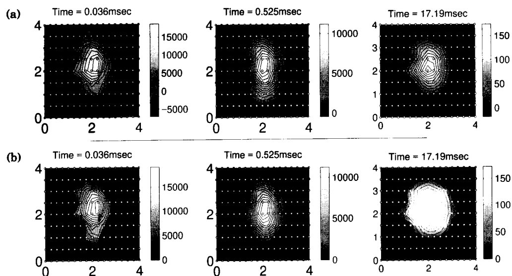
Figure 5.10: Removal of data that fall beneath the noise level. In the top set of panels (a), are the Z -component of the \partial \mathbf{B} / \partial t data, for three time channels. The bottom set of panels (b), have those data which fall beneath the noise level set by the \epsilon(t) = At^{-B} removed.
