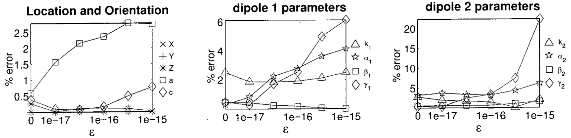
Figure 3.22: The recovered parameters for different choices of \epsilon . Recall that for this data set that the minimum amplitude datum was set to 1 \times 10^{-17} \text{V/m}^2 . Increases in \epsilon are reduces the accuracy with which we can recover the model parameters. The \gamma parameter is the most sensitive to changes in \epsilon .
