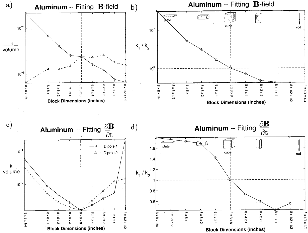
Figure 4.9: Relating the aspect ratio of an aluminum target with the ratio k_1/k_2 . Plot (a) contains the recovered k parameter when fitting the parameterization to the \mathbf{B} -field response obtained by integrating the \partial \mathbf{B}/\partial t response of an aluminum target. Plot (b) illustrates the relationship between the k_1/k_2 ratio and the shape of an aluminum target. Plot (c) contains the recovered k parameter from fitting the parameterization to the measured \partial \mathbf{B}/\partial t response. Plot (d) illustrates the relationship between the k_1/k_2 ratio and the shape of a aluminum target.
