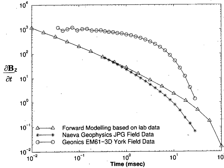
Figure 5.22: Comparison of \partial \mathbf{B} / \partial t response of a 105 mm shell. This plot includes the forward modelled response using parameters obtained from the Geonics Lab data ( \Delta ), the response measured above the UXO using the EM61-3D ( \circ ), and the response measured using a modified EM61 with a 5 m square transmitter loop ( * ) (obtained from Naeva Geophysics).
