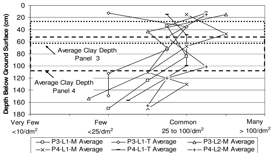
Figure 4: Mean rooting density versus depth in profile
