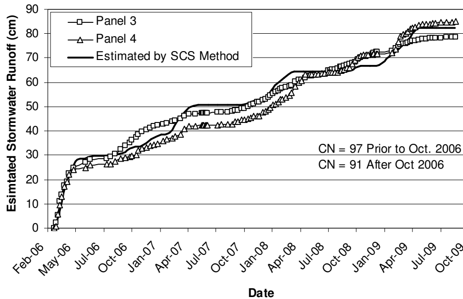
Figure 2: Simulated and observed stormwater runoff
