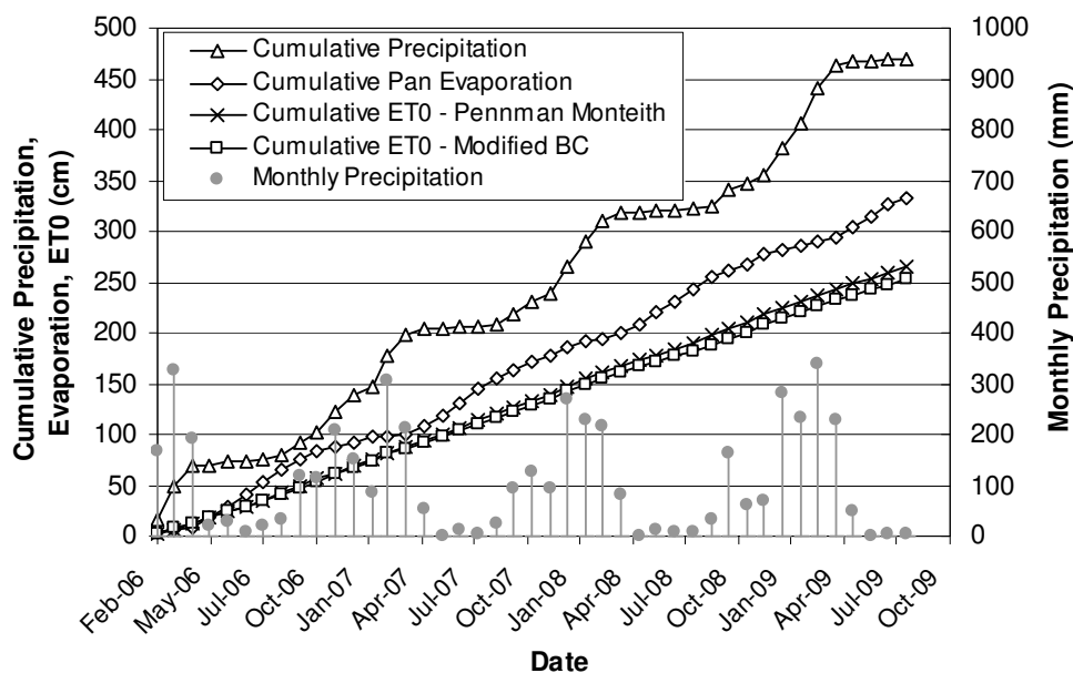
Figure 1: Estimated test panel precipitation, pan evaporation and predicted evapotranspiration
