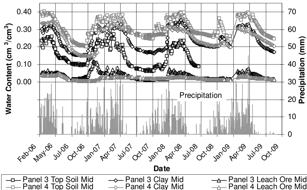
Figure 3: Side-slope middle area water content sensor data
