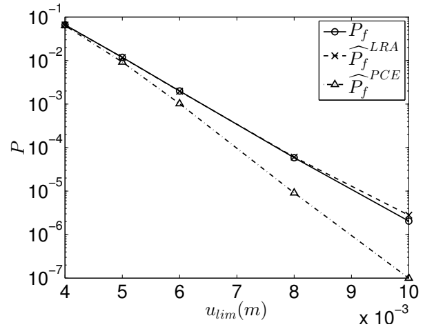
Figure 5: Comparison of failure probabilities evaluated with LRA and PCE to a reference value ( N = 50 ).
