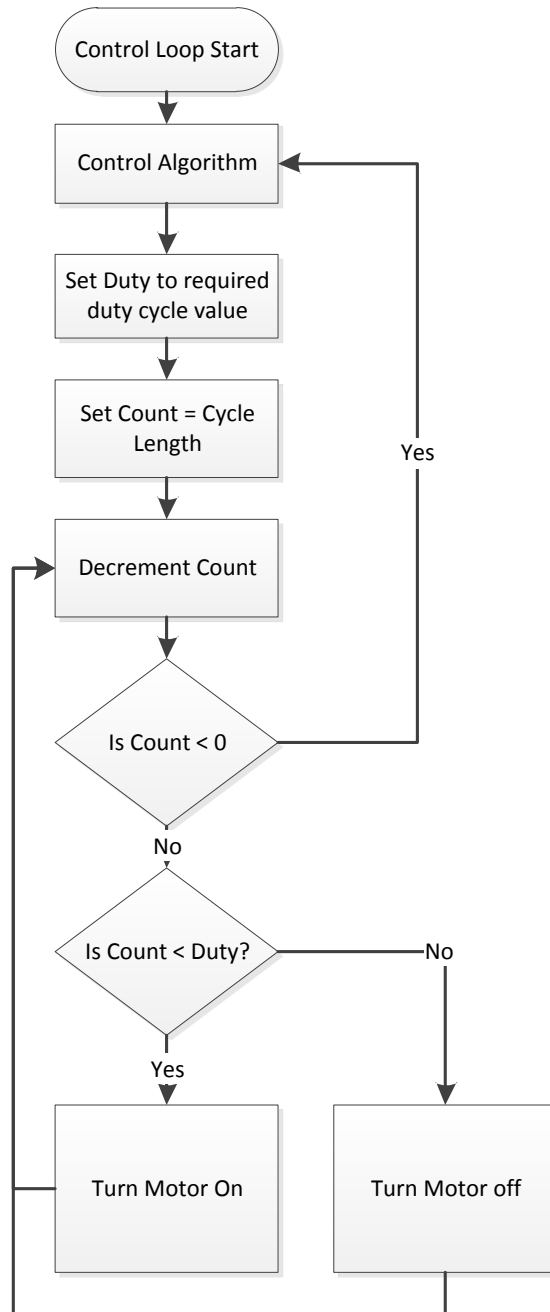
FIGURE 7: BLOCKING PWM
