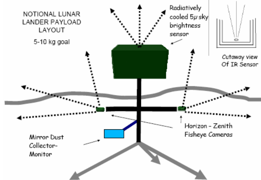
Fig 8. Design concept for a micro-Lander to conduct a site test at the pole. Sensors measure dust deposition and any thermal emission from a dust atmosphere above. Cameras view the terrain and sun around the horizon.
