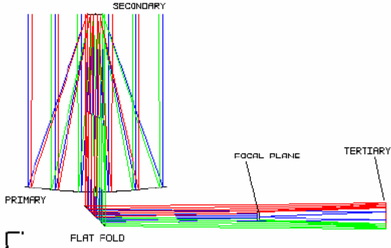
Fig 2. Three mirror telescope design by Dr. Simon Thibault.
