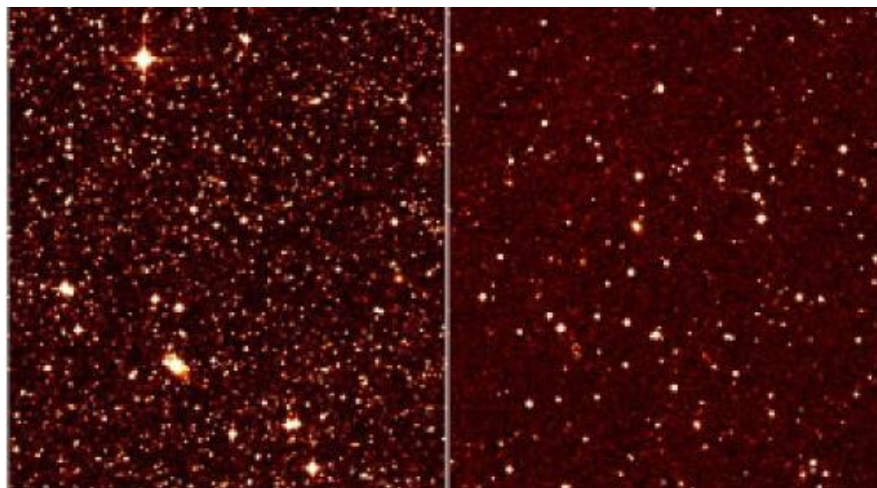
Fig 6. Comparison of N and S ecliptic poles. Schmidt survey photographic R-band images; Left - South Pole view, Right - North Pole view. R_{\text{limit}} = 21 ; FWHM = 2'' ; FOV = 12' \times 12' .
