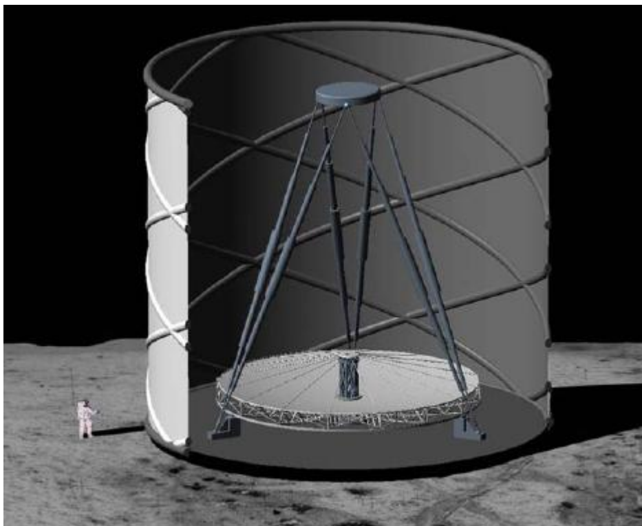
Fig 1. Artist's impression of the 20 m telescope. The secondary mirror is erected by extending the six telescoping legs, and the sunshield by inflation. The scientific instruments are below the bearing pier, shielded by lunar soil. (drawn by Tom Connors, University of Arizona).
