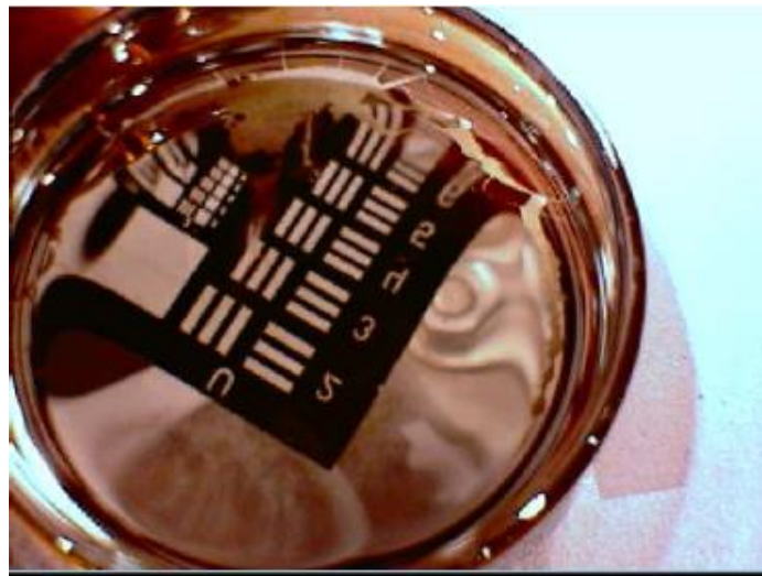
Fig 5. Mirror surface of silver on polypropylene glycol deposited by Ermanno Borra, University of Laval.
