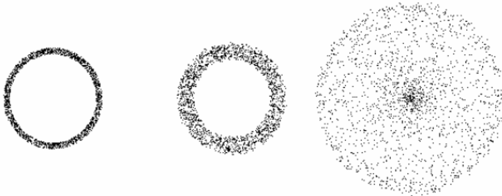
Fig 7. Effect of location on sky access for a zenith-pointed telescope with 0.2 degree field of view. The integrated exposure over 18 years is shown in each case. Left – at the pole, over 18.6 years the field sweeps out an annulus 3.1 degrees in diameter centered on the ecliptic pole, with continuous integration of ~ 5 months on any one spot. Center – 0.2 degrees from the pole, the field sweeps out a half degree annulus each month, covering any one spot every month for a year Right – 1.55 degrees from the pole. Each month the field sweeps a 3.1 degree annulus, covering any spot for about 15 hours. The ecliptic pole is seen for this time every month, for a total integration time of 5 months over 18 years.
