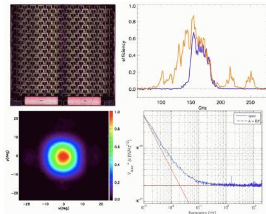
Figure 7. Top Left: A single 150 GHz pixel comprising a 288 element phased array of dual polarization slot antennas coupled to a matched load by a superconducting microstrip network. Microstrip band-defining filters and TES detectors are visible at bottom. Bottom Left: Measured beam pattern. The beam ellipticity is <1\% . Polarization efficiency is >98\% . The sidelobes ( <-13\text{dB} ) will be truncated at the 4K primary aperture stop. Top right: Measured spectra - orange and blue curves correspond to unfiltered and filtered antenna spectral response. Bottom right: Measured electrical NEP of a Ti TES. More on this can be found in Kuo et al. in this proceeding[5].
