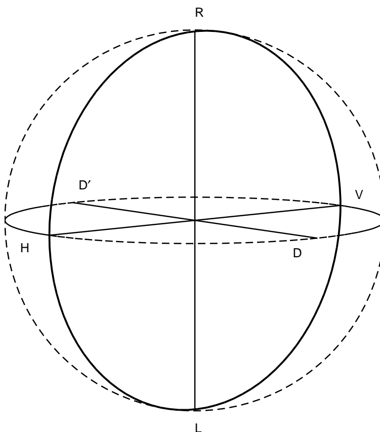
Figure 1. 3-D perspective view of the Poincaré sphere showing several special polarization states. The H and V points correspond to horizontal and vertical linear polarizations. The R and L points correspond to right and left circularly polarized light. The D and D' points correspond to linearly polarized light at \pm 45 degrees to the horizontal. The HRVL circle is emphasised.
