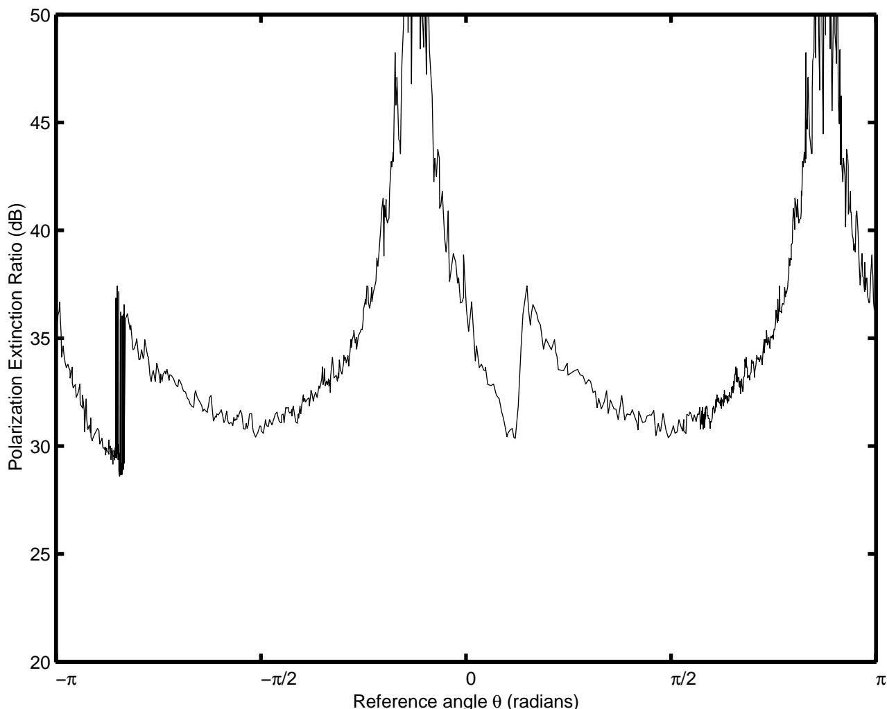
Figure 8. Maximum polarization extinction ratio as a function of the reference angle \theta , defined in Figure 7c.
