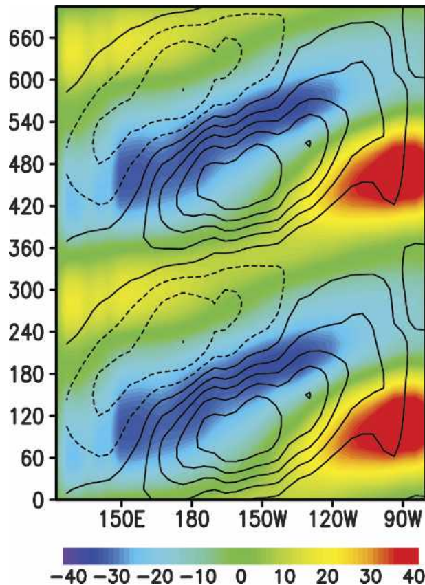
FIG. 5. Phase-longitude section of the thermocline anomaly (in color: m) and the zonal wind stress anomaly (in contour: \times 10^{-1} \text{ N m}^{-2} ) along the equator ( 5^{\circ}\text{S} – 5^{\circ}\text{N} ) associated with the first mode NLPCA. Phase in the y axis represents the time sequence. Two cycles are plotted with the phase (in ^{\circ} ) increasing with time. Contour interval is 0.1 \text{ N m}^{-2} .
