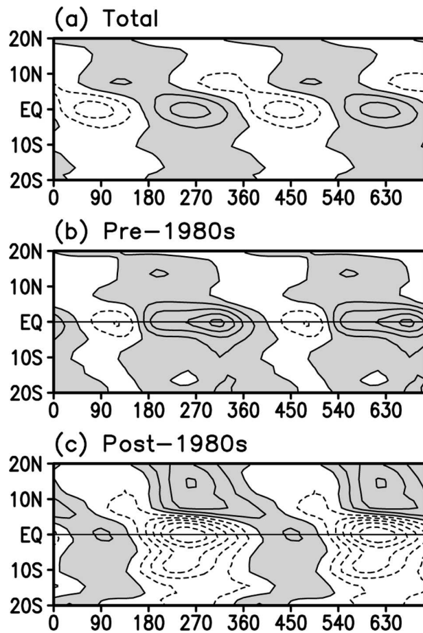
FIG. 9. Phase-latitude section of the zonal-mean thermocline anomaly associated with the first mode NLPFA for (a) the total period, (b) pre-1980s only, and (c) post-1980s only. Contour interval is 4 m. Positive values are shaded.
