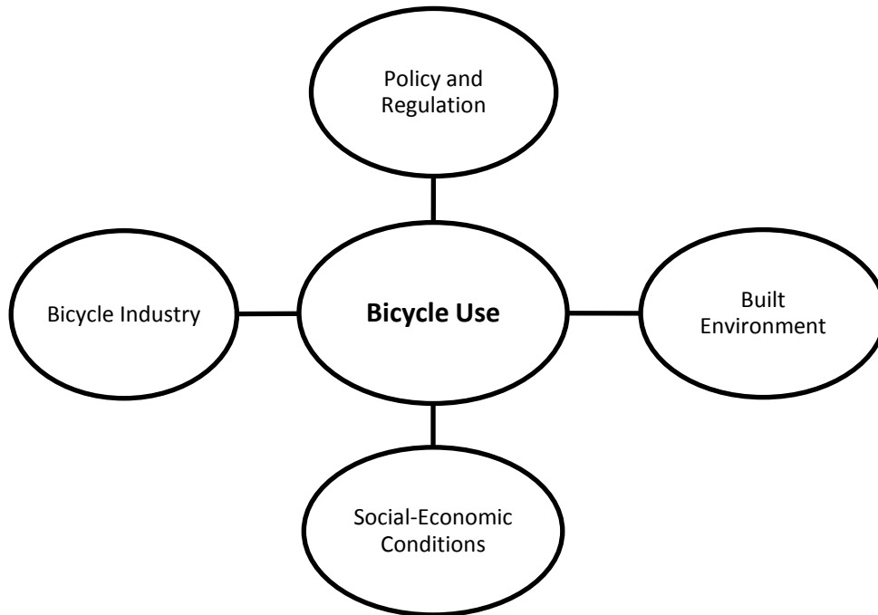
Figure 2: Analytical Framework
