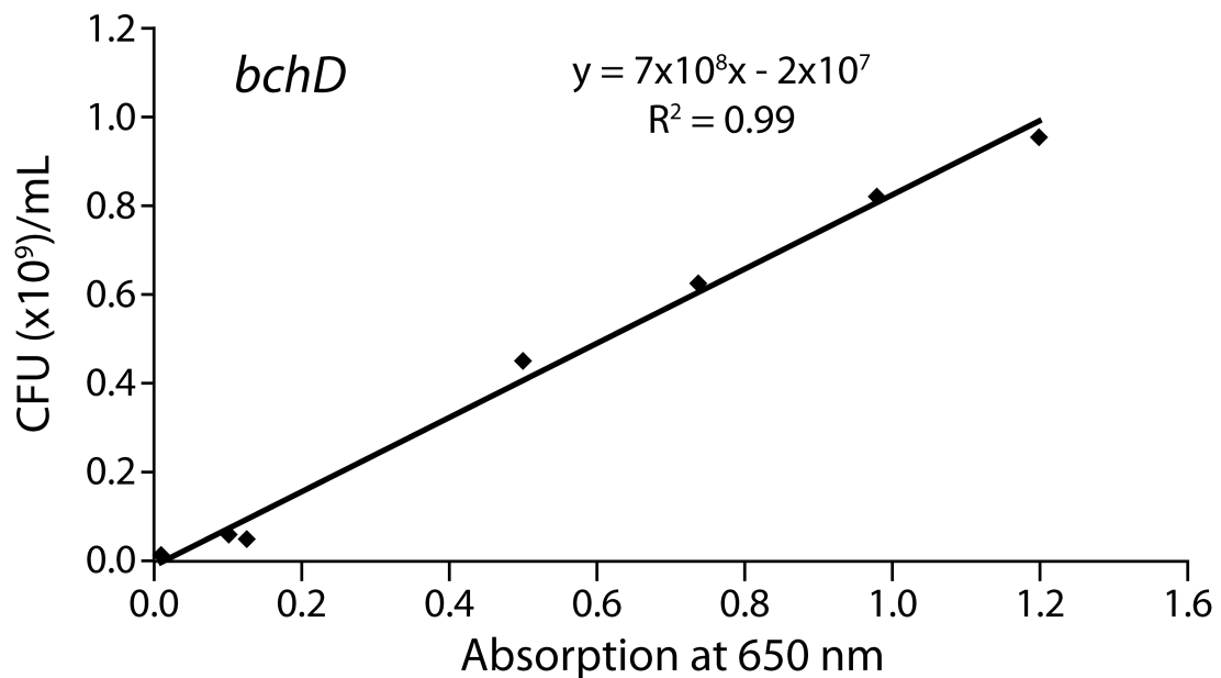
Figure AI. Comparison of numbers of CFUs per unit of absorbed light at 650 nm in wt and bchD mutant. (A) Wild type. (B) bchD mutant. Samples were taken from cultures growing semiaerobically, diluted and spread on LB plates, then colonies were counted after three days of growth at 30°C.
