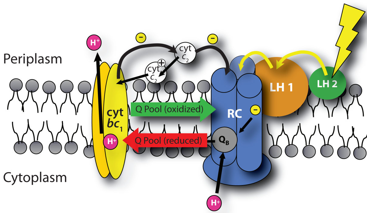
Figure 1-4. Light-driven cyclic electron transfer of the Rb. sphaeroides photosynthetic apparatus imbedded in a lipid bilayer. H^+ , protons; - , electrons; RC, reaction center; cyt\ bc_1 , cytochrome bc_1 complex; cyt\ c_2 , cytochrome c_2 protein; LH1, light-harvesting 1 complex; LH2, light-harvesting 2 complex; Q_B , quinone/quinol; yellow arrow, exciton energy transfer; red and green arrows represent the flow of quinone molecules between the RC and cyt\ bc_1 complexes.
