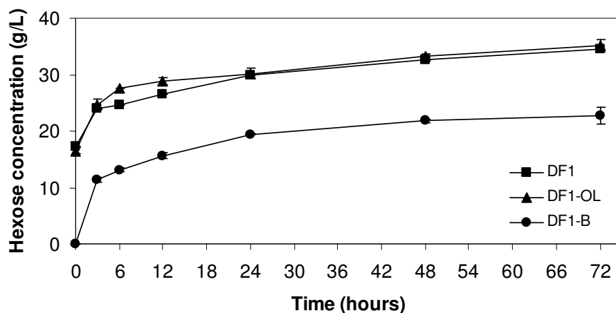
Figure 3-25. Enzymatic hydrolysis of DF1 water-insoluble fraction in water soluble fraction, overlimed water soluble fraction and pH 4.8 acetate buffer at 5% consistency (w/v) with 40 FPU/g glucan (Spezyme) and \beta -glucosidase at 40 CBU/g glucan (Novozymes 188). (DF1: DF1 water soluble fraction; DF1-OL: overlimed DF1 water soluble fraction; DF1-B: pH 4.8 acetate buffer) Error bars denote standard deviations.
