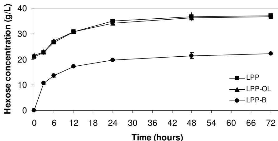
Figure 3-27. Enzymatic hydrolysis of LPP water-insoluble fraction in water soluble fraction, overlimed water soluble fraction and pH 4.8 acetate buffer at 5% consistency (w/v) with 40 FPU/g glucan (Spezyme) and \beta -glucosidase at 40 CBU/g glucan (Novozymes 188). (LPP: LPP water soluble fraction; LPP-OL: overlimed LPP water soluble fraction; LPP-B: pH 4.8 acetate buffer) Error bars denote standard deviations.
