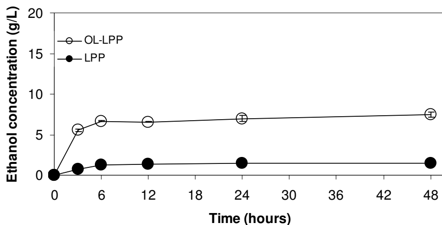
Figure 3-20. Ethanol production (g/L) by yeast strain T2 from fermentation of steam-pretreated LPP water soluble fraction with and without overliming treatment. Error bars denote standard deviations.
