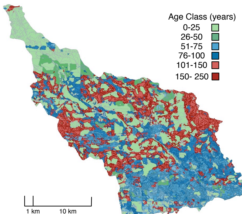
Figure 2.1: A region of forest in British Columbia with 1880 cells. Each colour indicates the dominant age class, in years, of trees in the cell.
